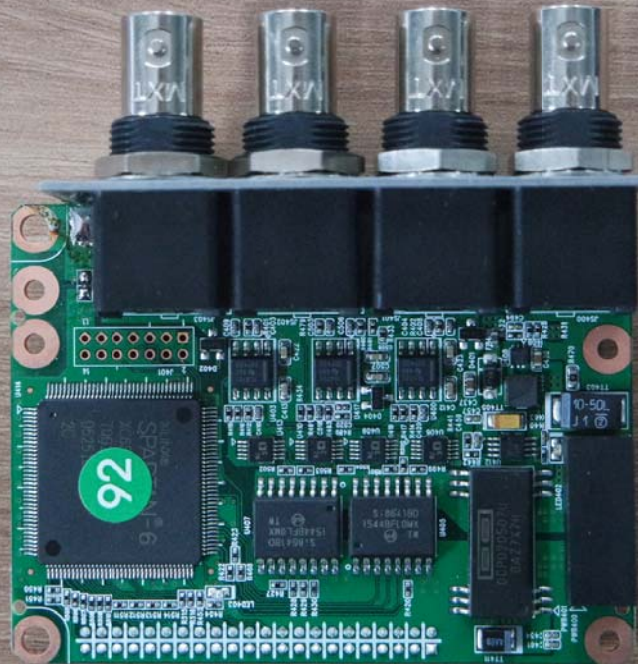
Sensor Board PCB - Rear
