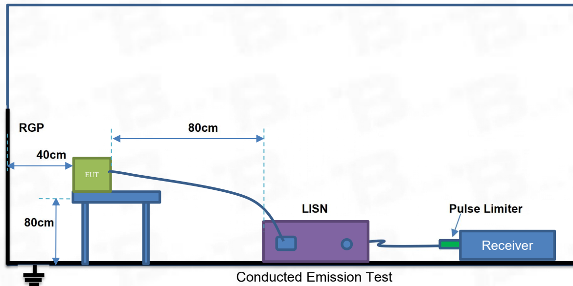
Test Setup 2
