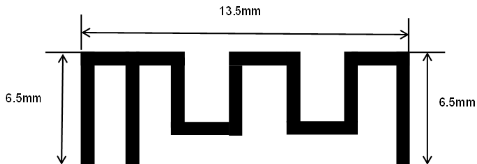
Antenna Photo&Length
