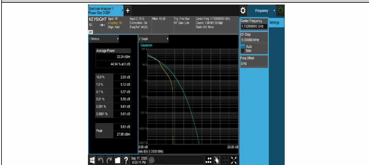
Band4-3MHz-16QAM-20175-15RB#0
