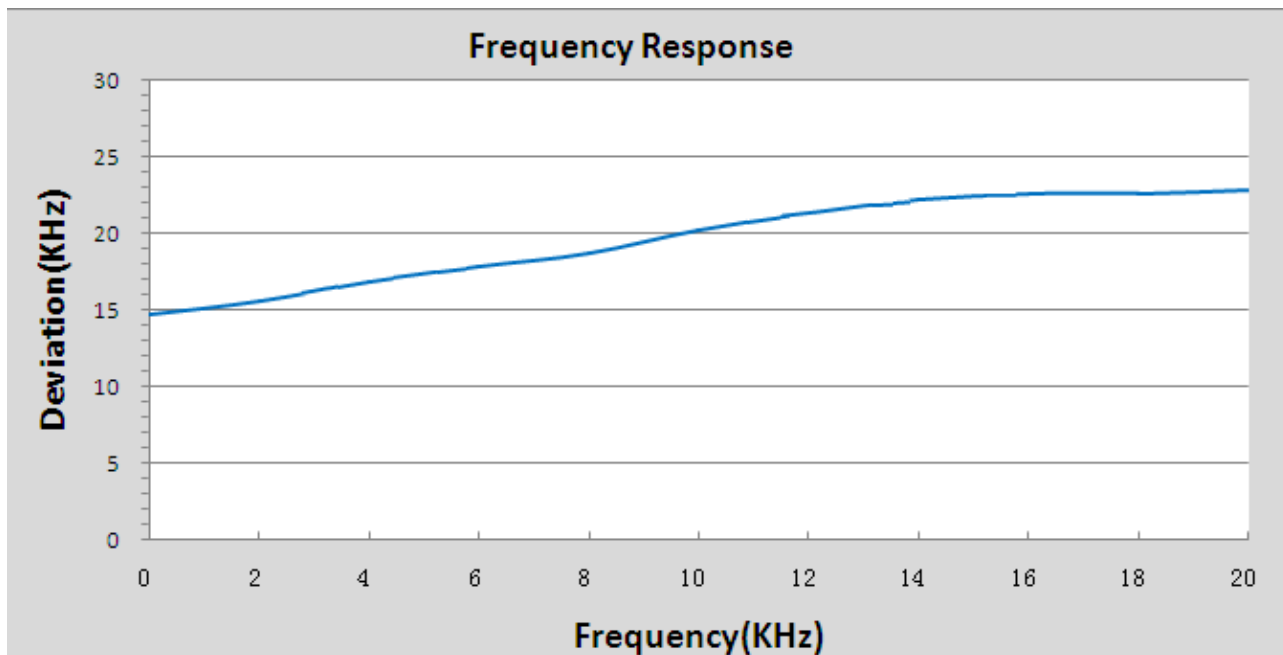
520MHz Channel
