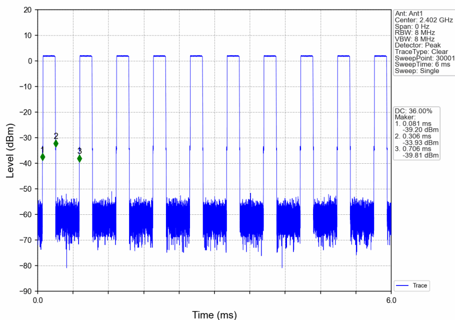
2M_LCH_2402MHz_Ant1_NTNV
