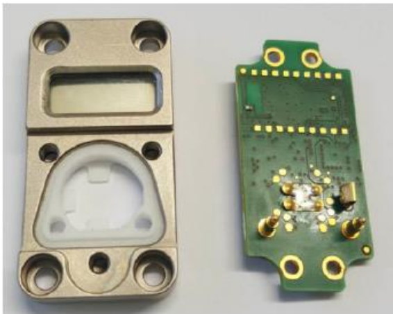
Mechanical Lid and PCB Top
