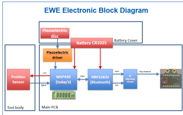
Picture 3. Electronic Block Diagram.
