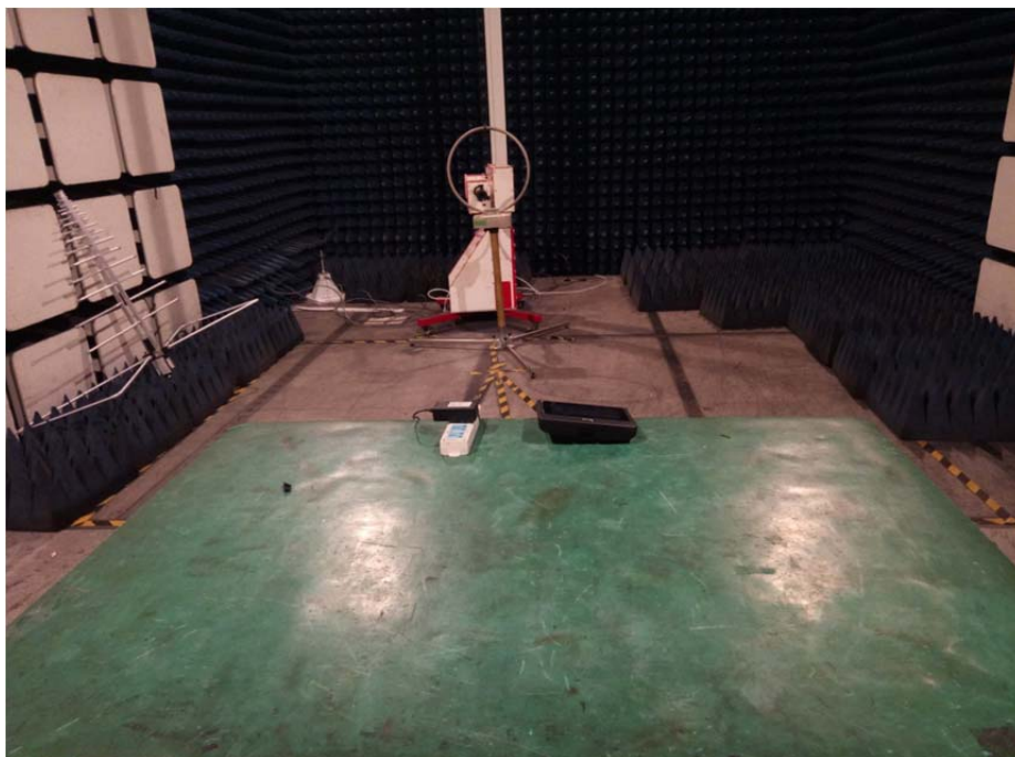
Spurious Emission
