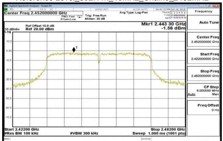
Reference Level_802.11n_40MHz_Chain0_2452MHz
