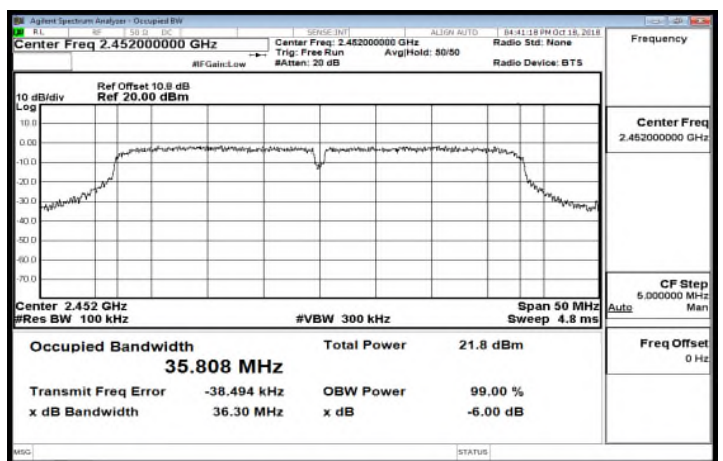
OBW 6dB_802.11n_40MHz_Chain0_2452MHz
