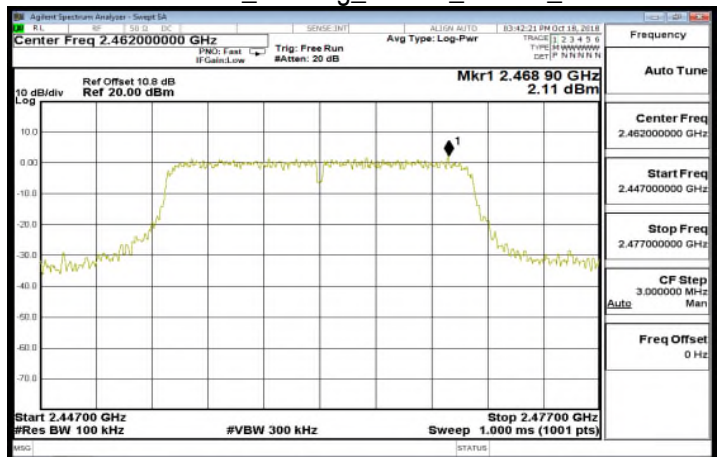
Reference Level_802.11g_20MHz_Chain0_2462MHz
