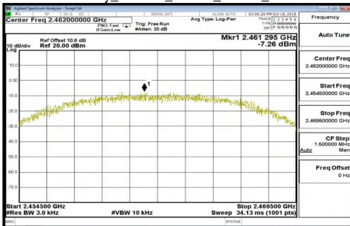
Power Density_802.11b_20MHz_Chain0_2462MHz
