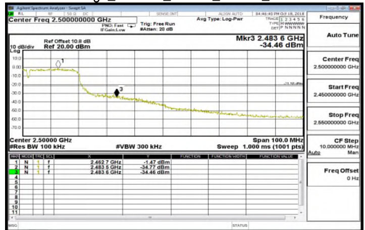
Band Edge_802.11n_40MHz_Chain0_2452MHz
