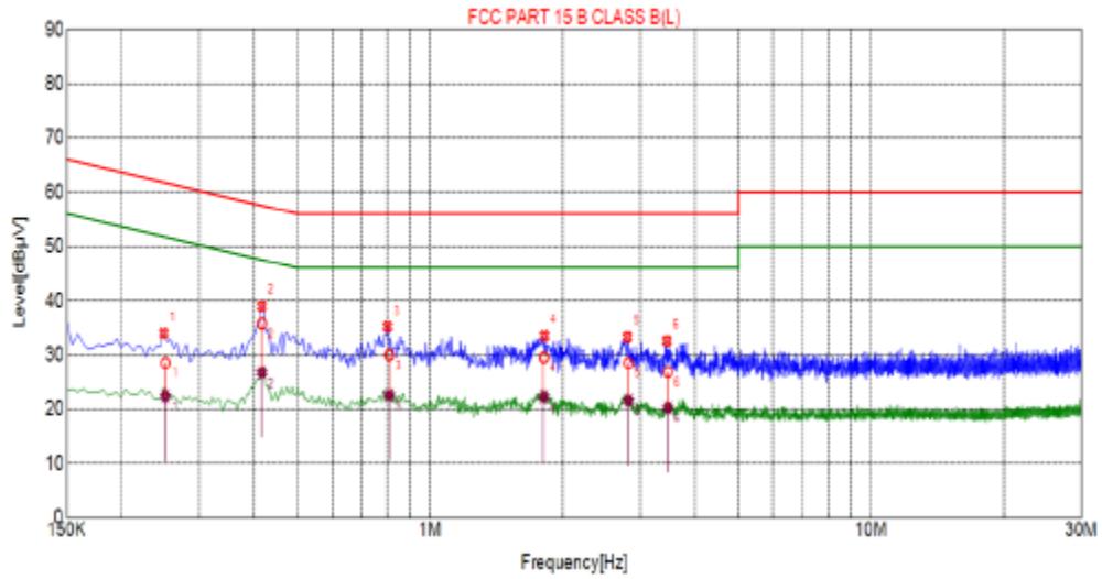
Line Conducted Emission Test Line 1-L
