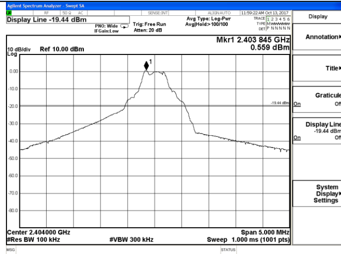
Channel 1 / 2404 MHz
