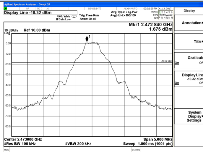
Channel 16 / 2473 MHz
