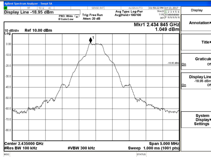
Channel 8 / 2435 MHz
