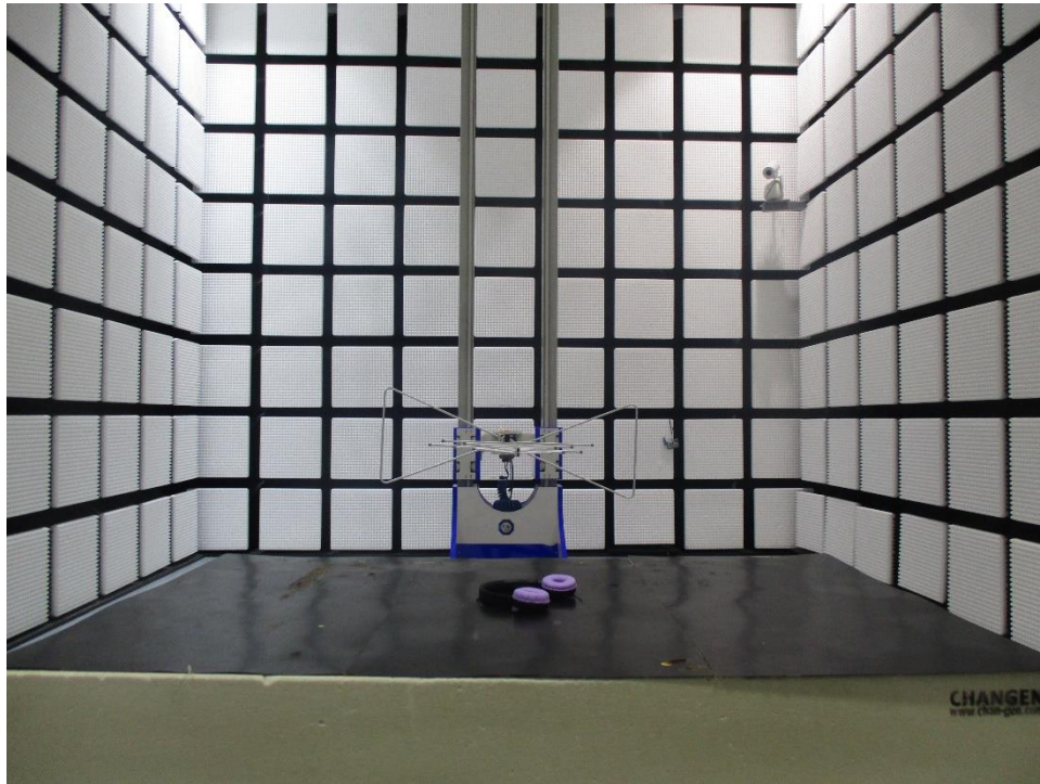
Spurious radiated below 1GHz
