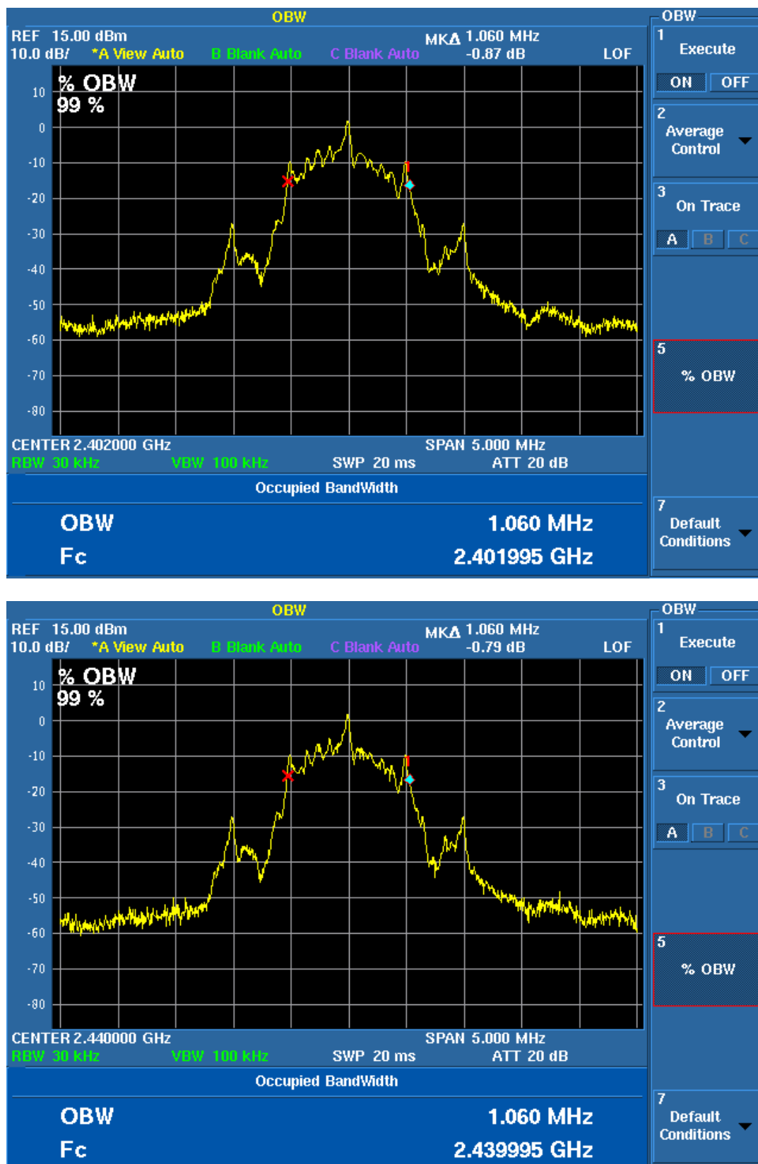
Figure 2. Occupied Bandwidth Plots
