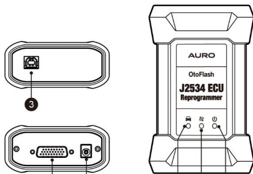
Figure 2-4 OtoFlash Views
