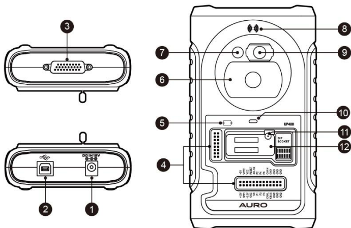
Figure 2-5 UP400 Views
