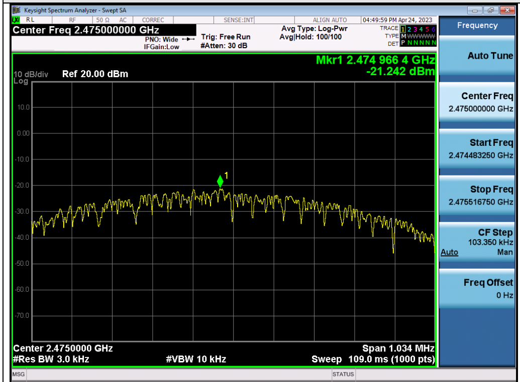
Test_Graph_2.4G_ANT1_2475_GFSK_PSD
