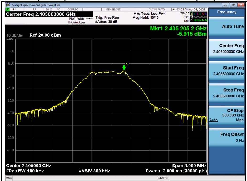
Test_Graph_2.4G_ANT1_2405_GFSK_Reference Level
