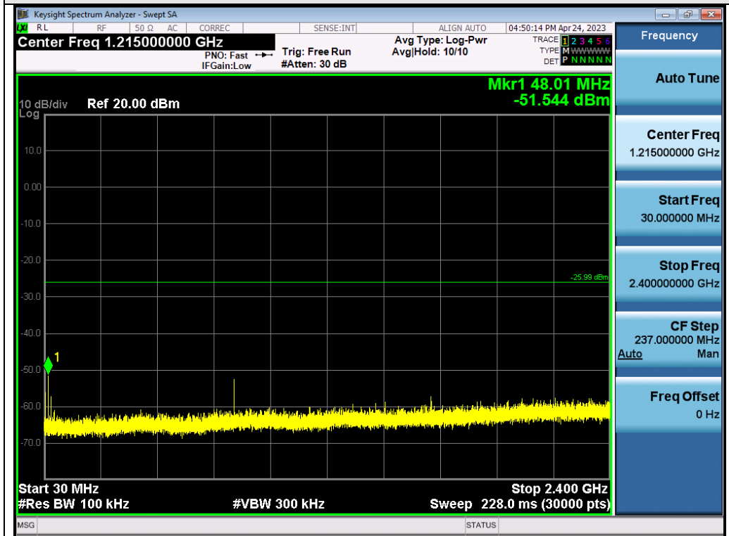
Test_Graph_2.4G_ANT1_2475_GFSK_Lower Band Emissions
