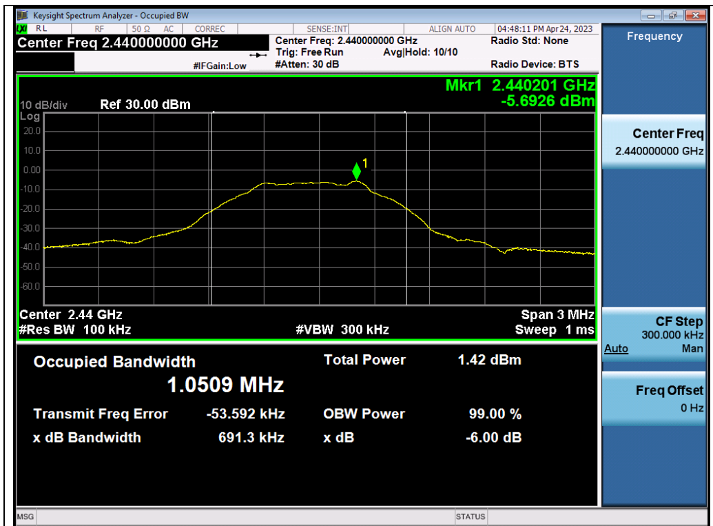
Test_Graph_2.4G_ANT1_2440_GFSK_DTSBW
