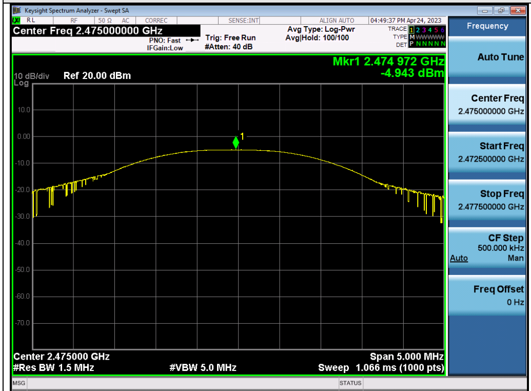
Test_Graph_2.4G_ANT1_2475_GFSK_Peak Power
