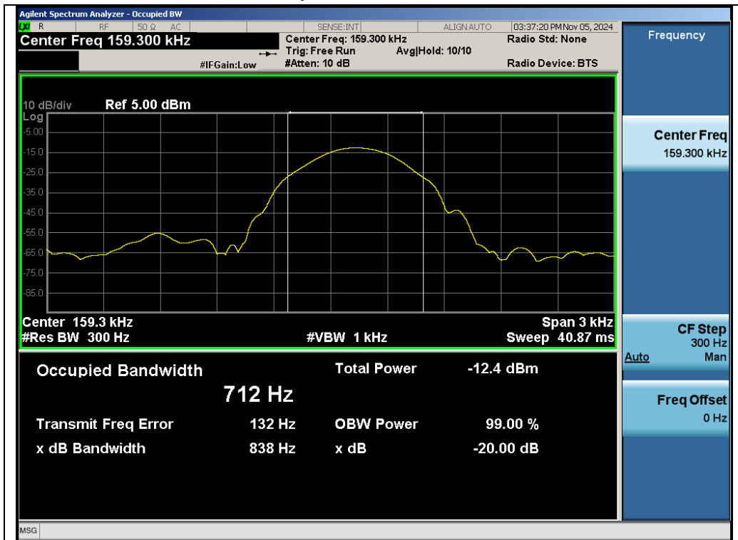
Test_Graph_ASK_Coil 1 st _159.3kHz_-20dB Bandwidth
