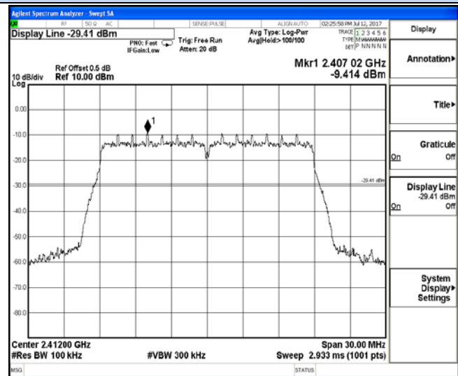
2397 MHz – 2427 MHz
