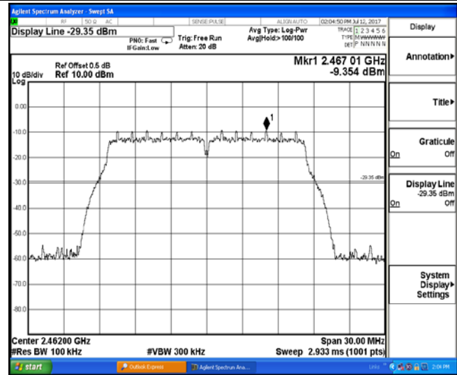
2447 MHz – 2477 MHz
