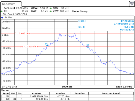
DH1_High 0.925MHz
