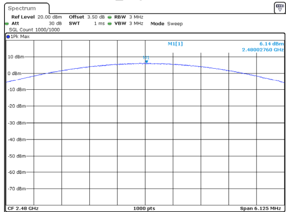
3DH1_High 6.14dBm
