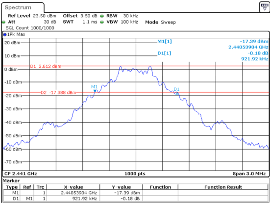
DH1_Middle 0.922MHz
