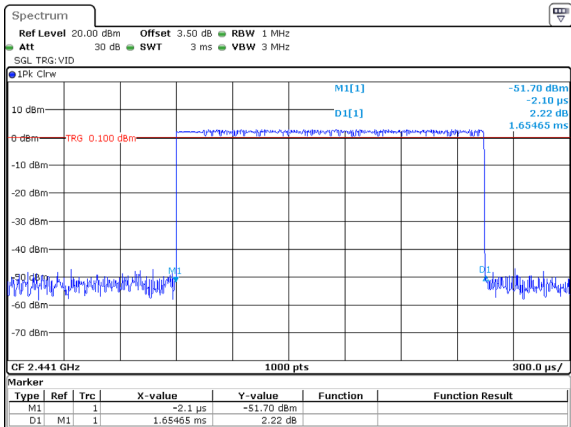
2DH3_Hopping 1.655ms
