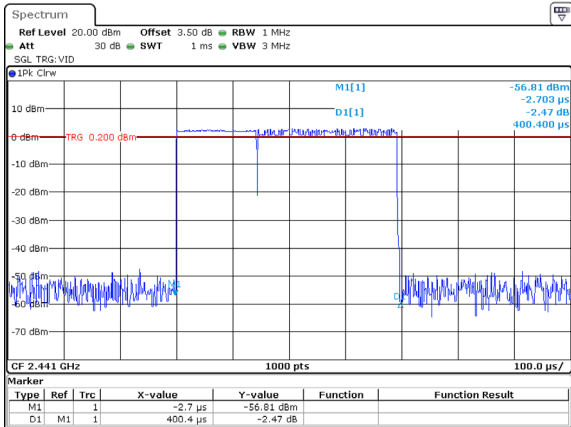
2DH1_Hopping 0.400ms
