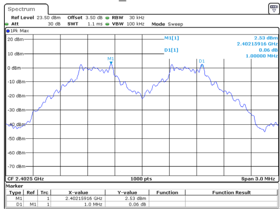
DH1_Low 1MHz
