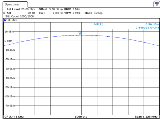
3DH1_Middle 6.36dBm
