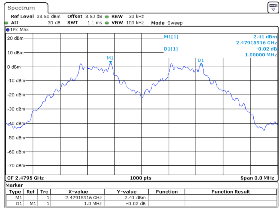
DH1_High 1MHz
