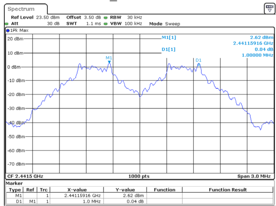
DH1_Middle 1MHz
