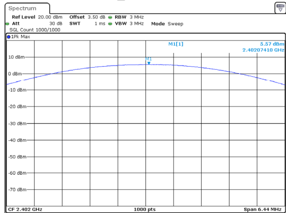
2DH1_Low 5.57dBm
