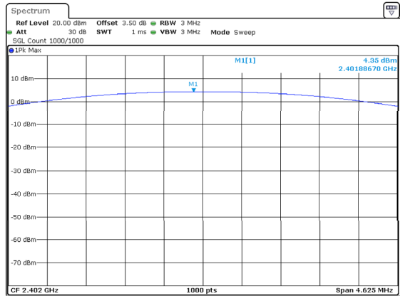
DH1_Low 4.35dBm
