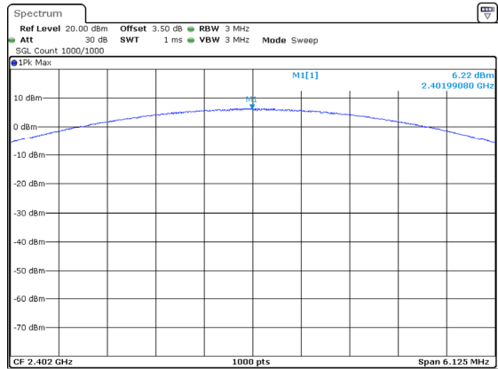
3DH1_Low 6.22dBm
