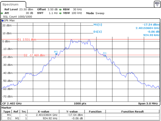
DH1_Low 0.925MHz
