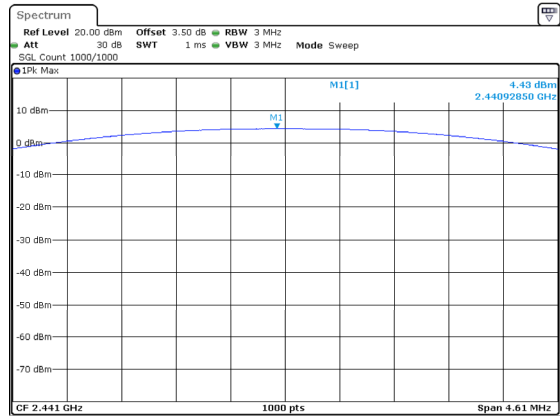
DH1_Middle 4.43dBm
