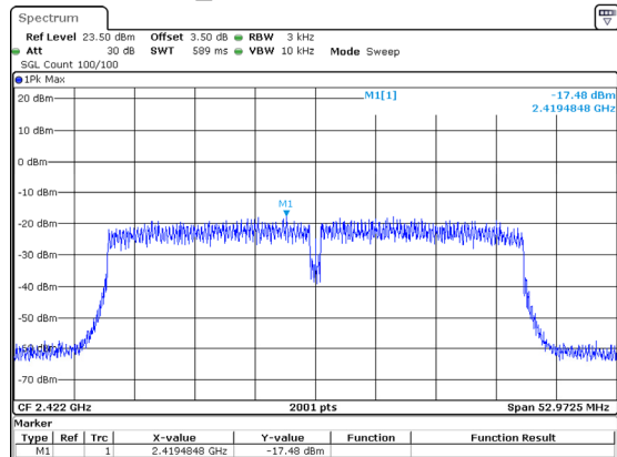
802.11n40_2422MHz -17.48dBm/3kHz
