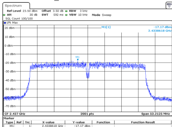
802.11n40_2437MHz -17.17dBm/3kHz
