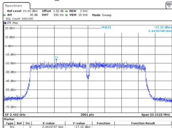
802.11n40_2452MHz -17.12dBm/3kHz
