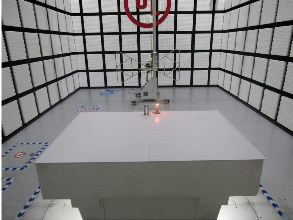
Radiated Disturbance below 1 GHz test setup photo
