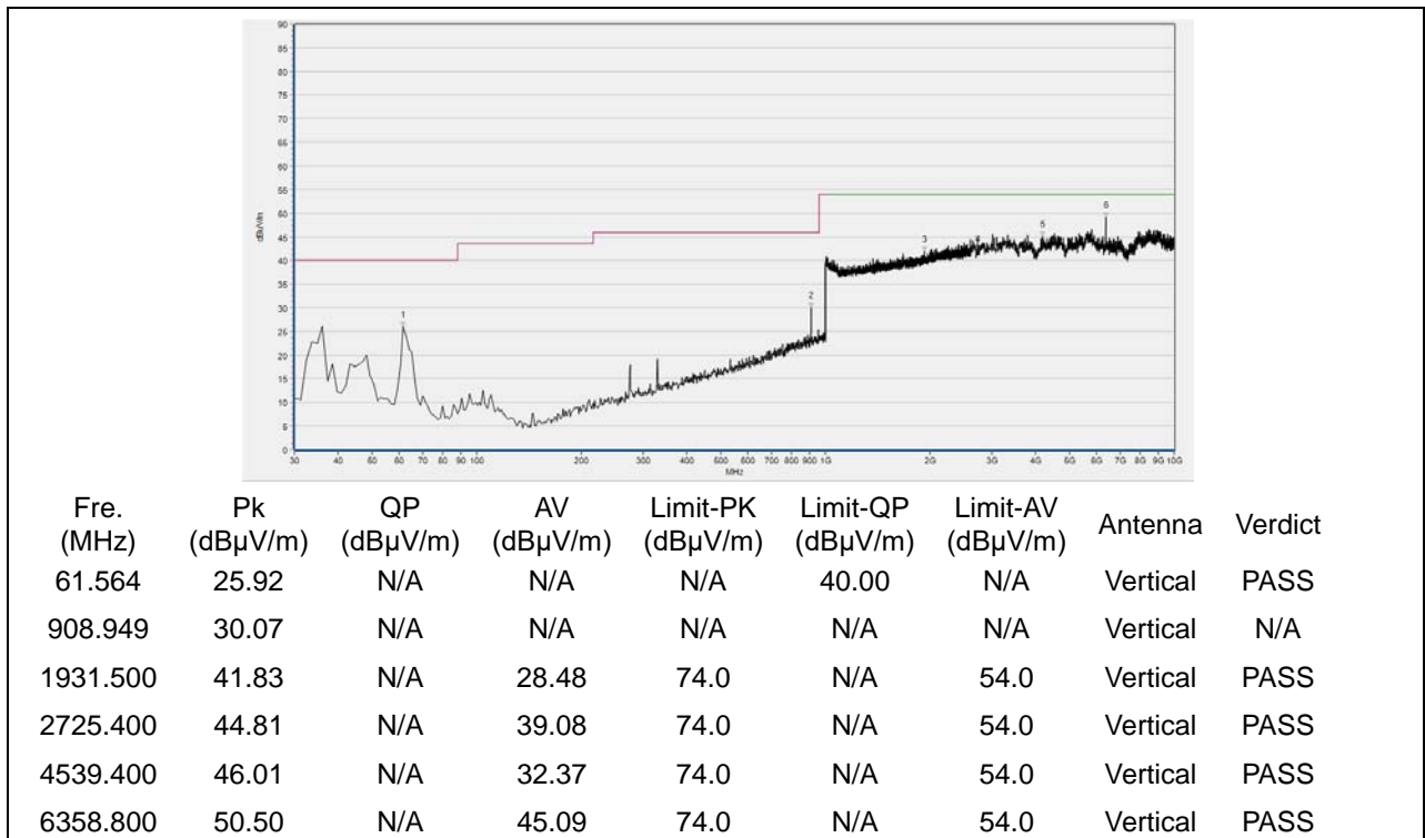
(908.4MHz, Antenna Vertical, 30MHz to 10GHz)
