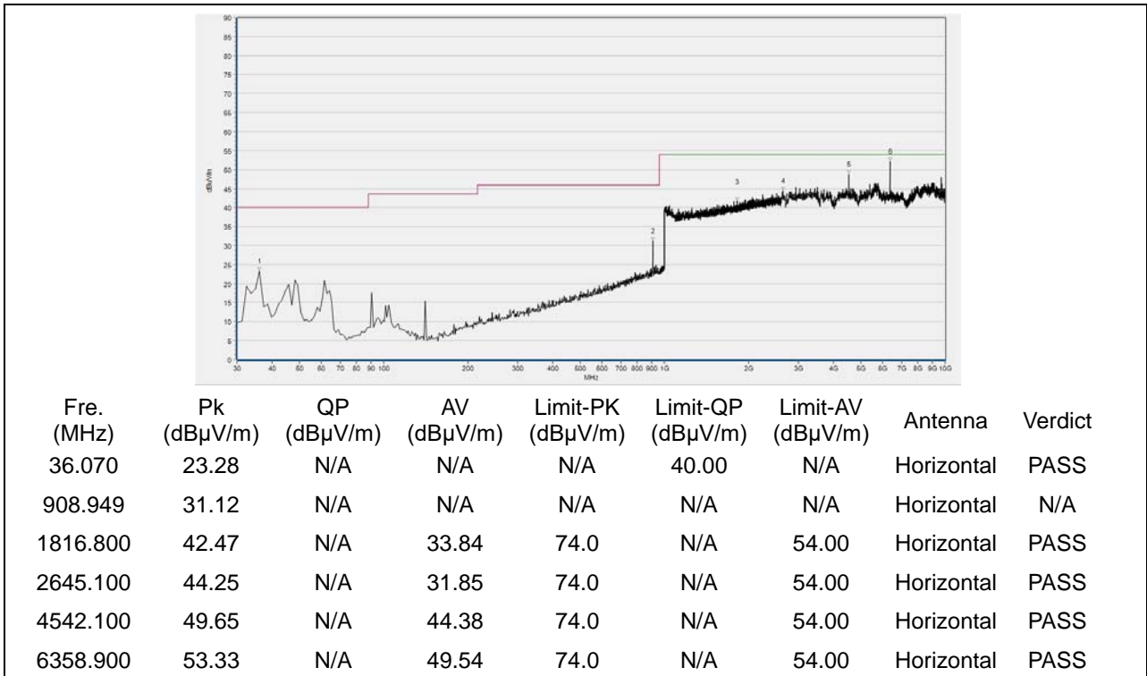
(908.4MHz, Antenna Horizontal, 30MHz to 10GHz)
