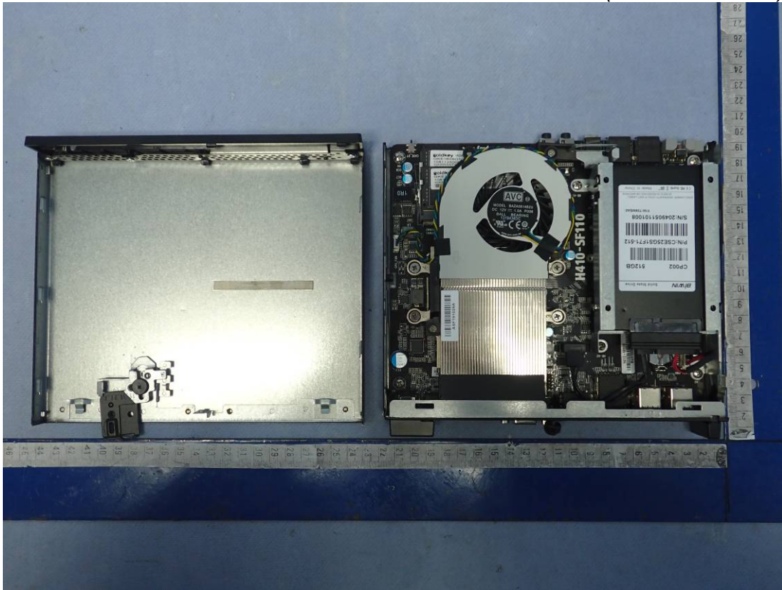
Figure 19 Case A Internal View (Removed Cover)
