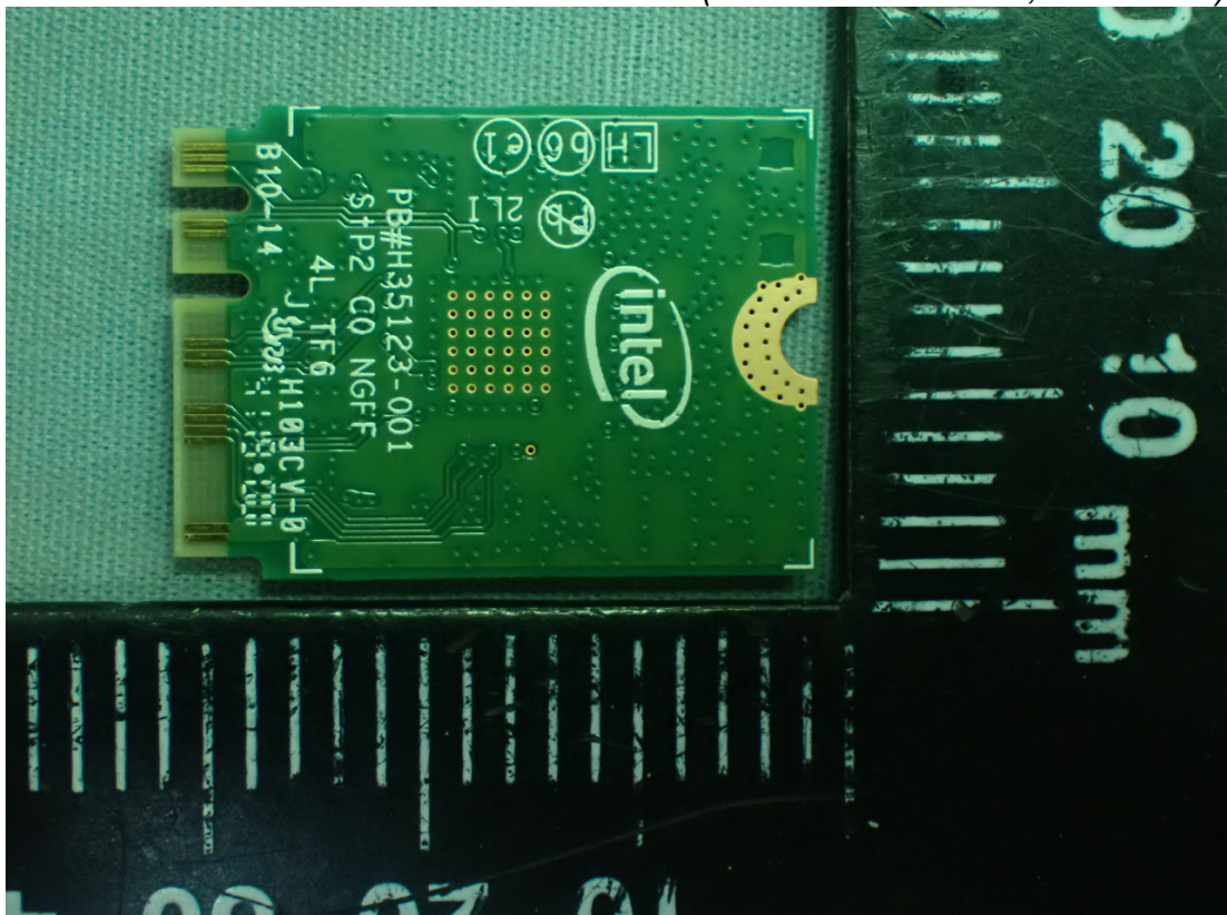
Figure 32 Internal View (WLAN Combo Card, Back View)
