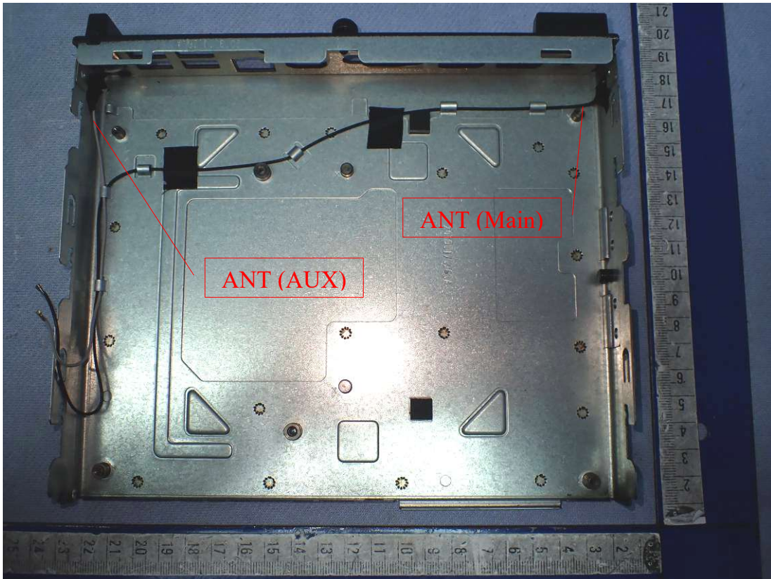
Figure 20 Case A Internal View
