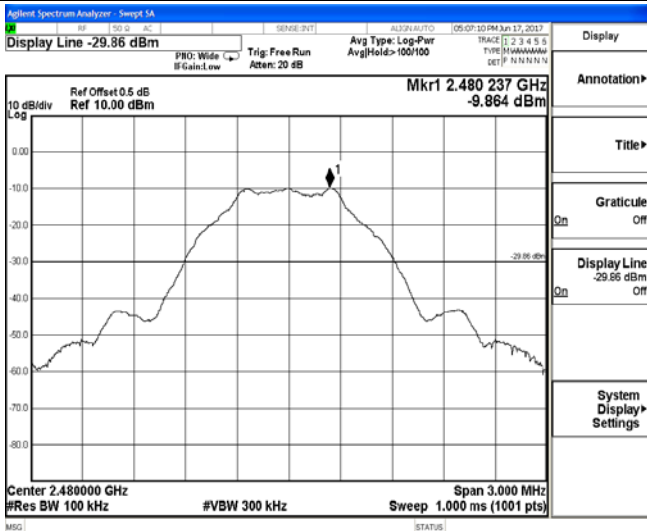
2479 MHz – 2481 MHz
