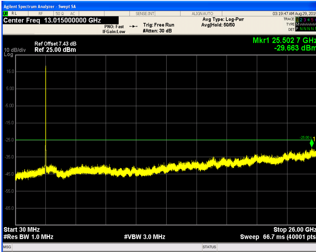
LTE Band41 QPSK BW=15MHz Channel=41115 RB Size=75 Position=#0
