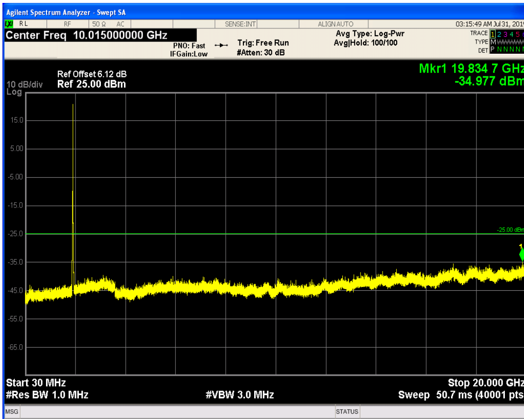
LTE Band1 QAM16 BW=15MHz Channel=18525 RB Size=75 Position=#0
