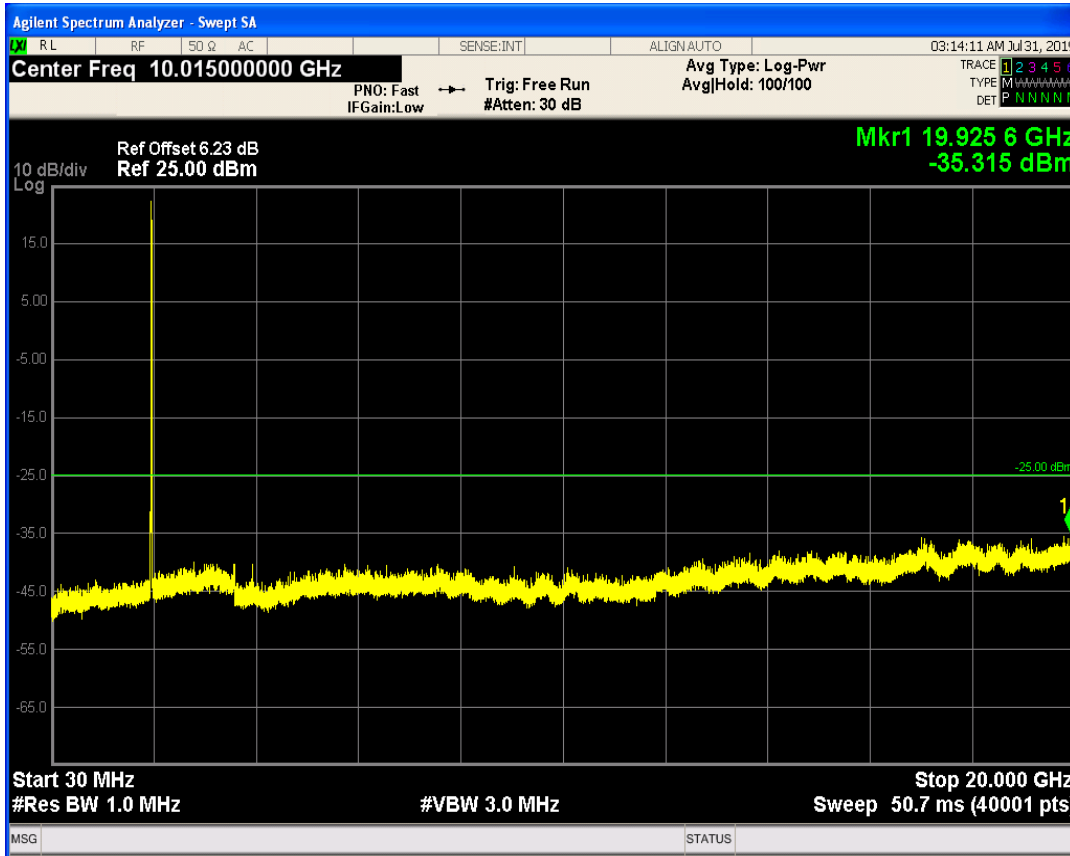
LTE Band1 QPSK BW=15MHz Channel=18075 RB Size=75 Position=#0
