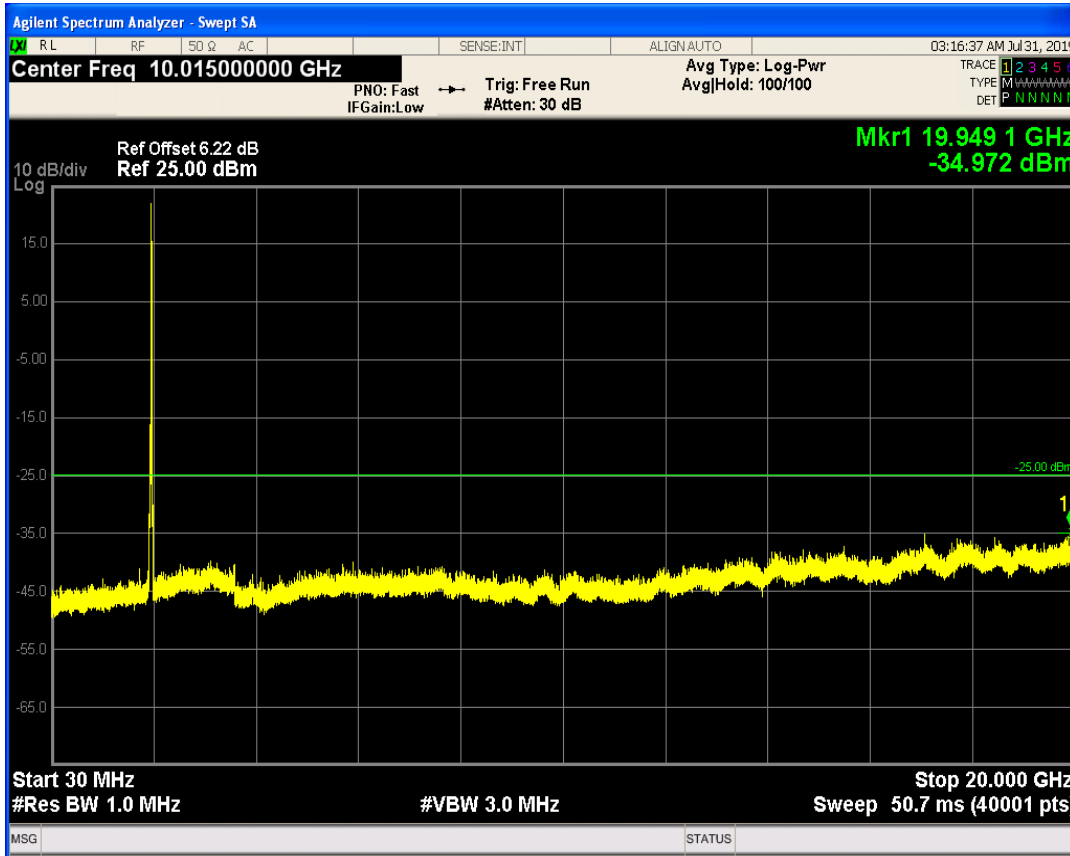
LTE Band1 QPSK BW=10MHz Channel=18050 RB Size=50 Position=#0
