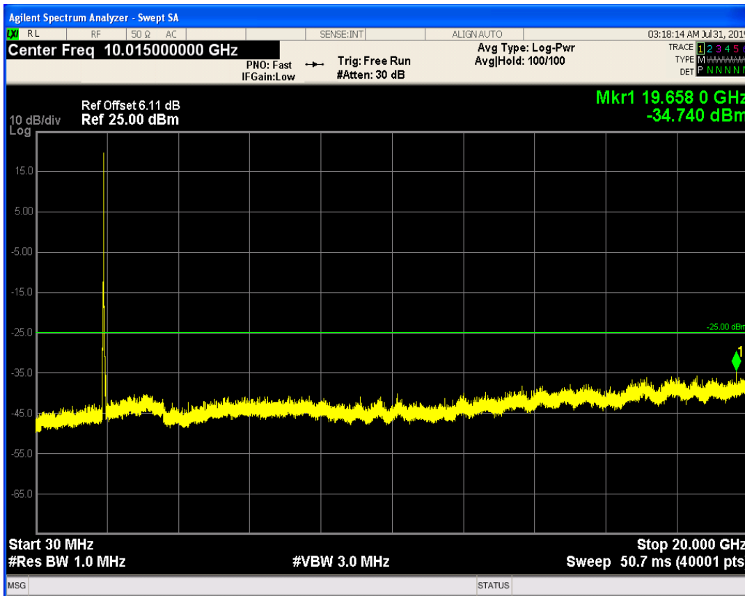
LTE Band1 QPSK BW=20MHz Channel=18500 RB Size=100 Position=#0
