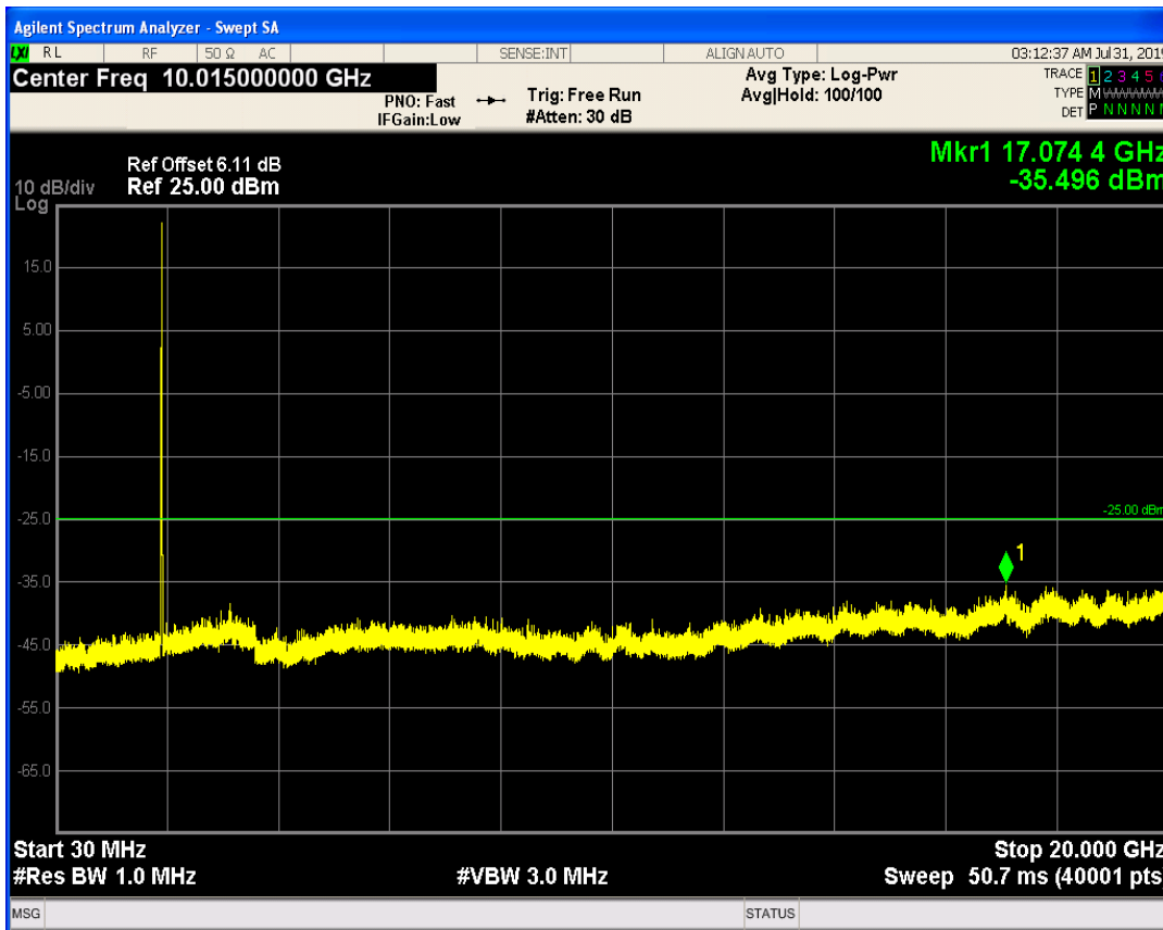
LTE Band1 QAM16 BW=20MHz Channel=18500 RB Size=100 Position=#0
