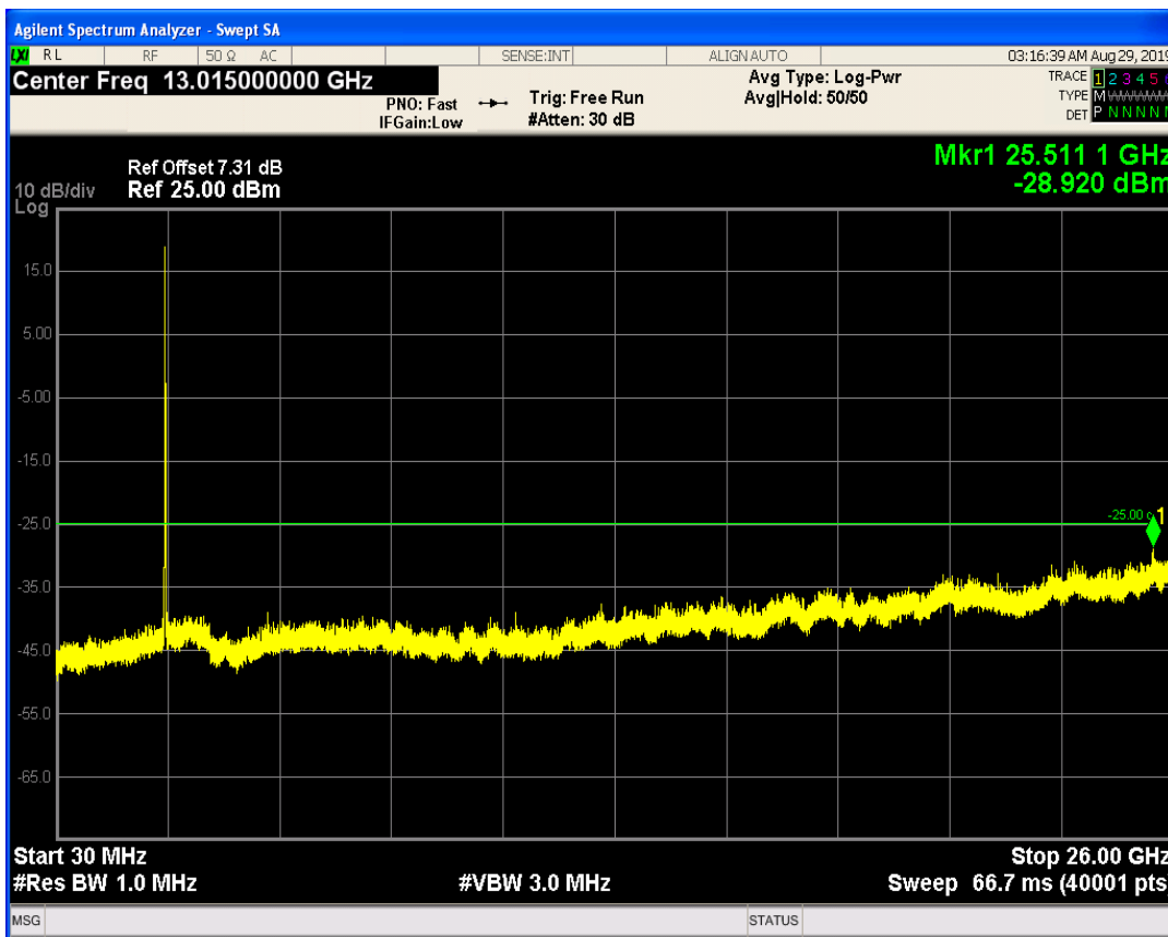
LTE Band41 QPSK BW=10MHz Channel=41140 RB Size=50 Position=#0
