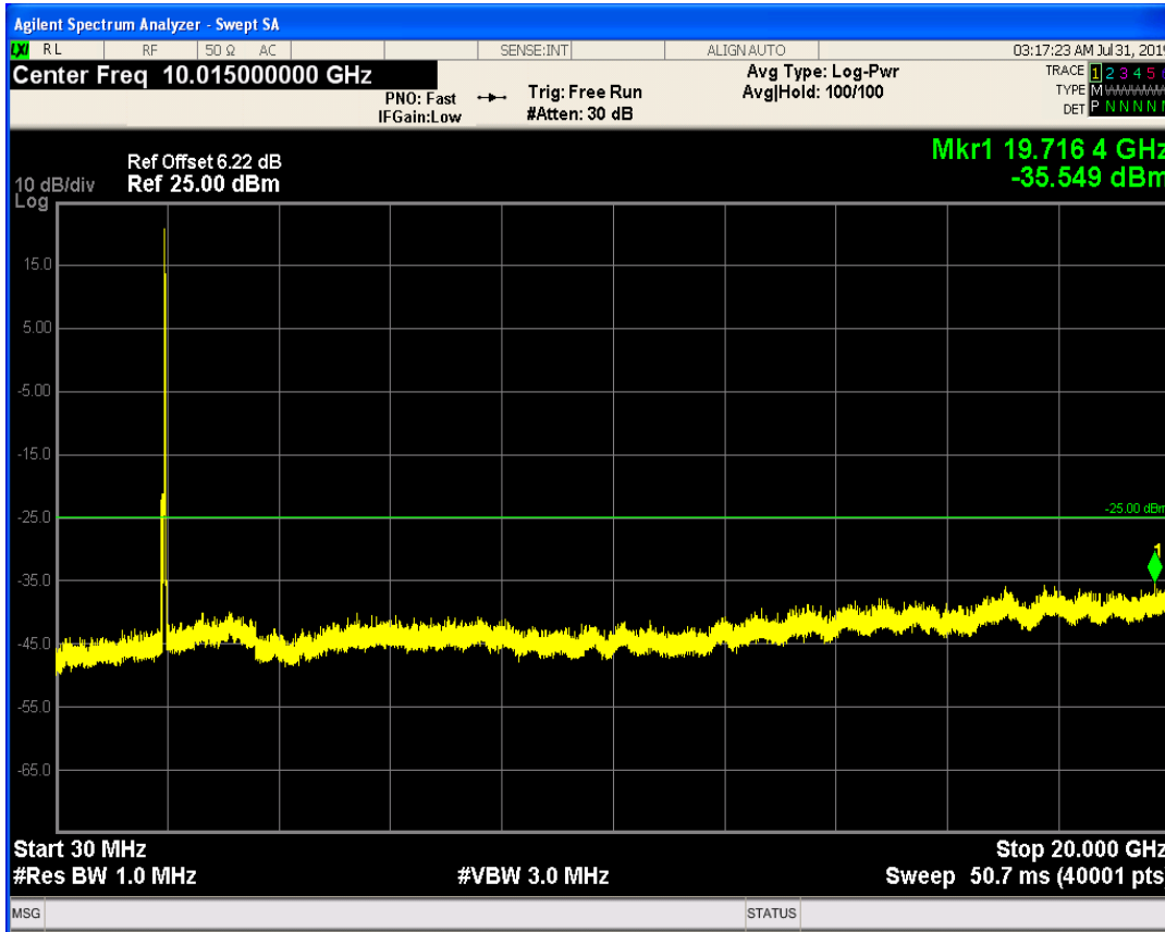
LTE Band1 QAM16 BW=10MHz Channel=18050 RB Size=50 Position=#0
