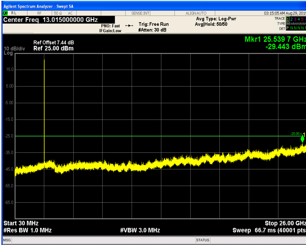
LTE Band41 QAM16 BW=5MHz Channel=41165 RB Size=25 Position=#0
