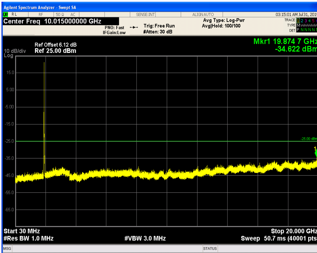
LTE Band1 QAM16 BW=5MHz Channel=18575 RB Size=25 Position=#0
