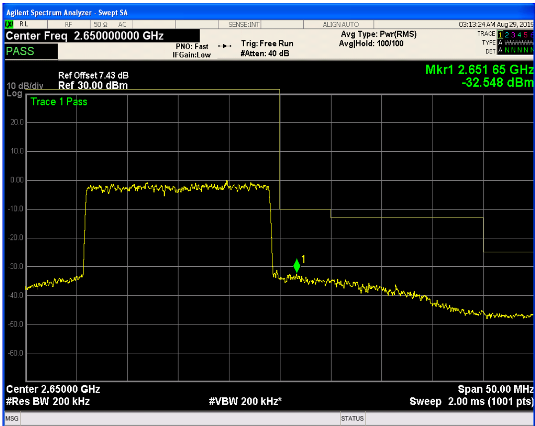
LTE Band41 QAM16 BW=20MHz Channel=41090 RB Size=100 Position=#0
