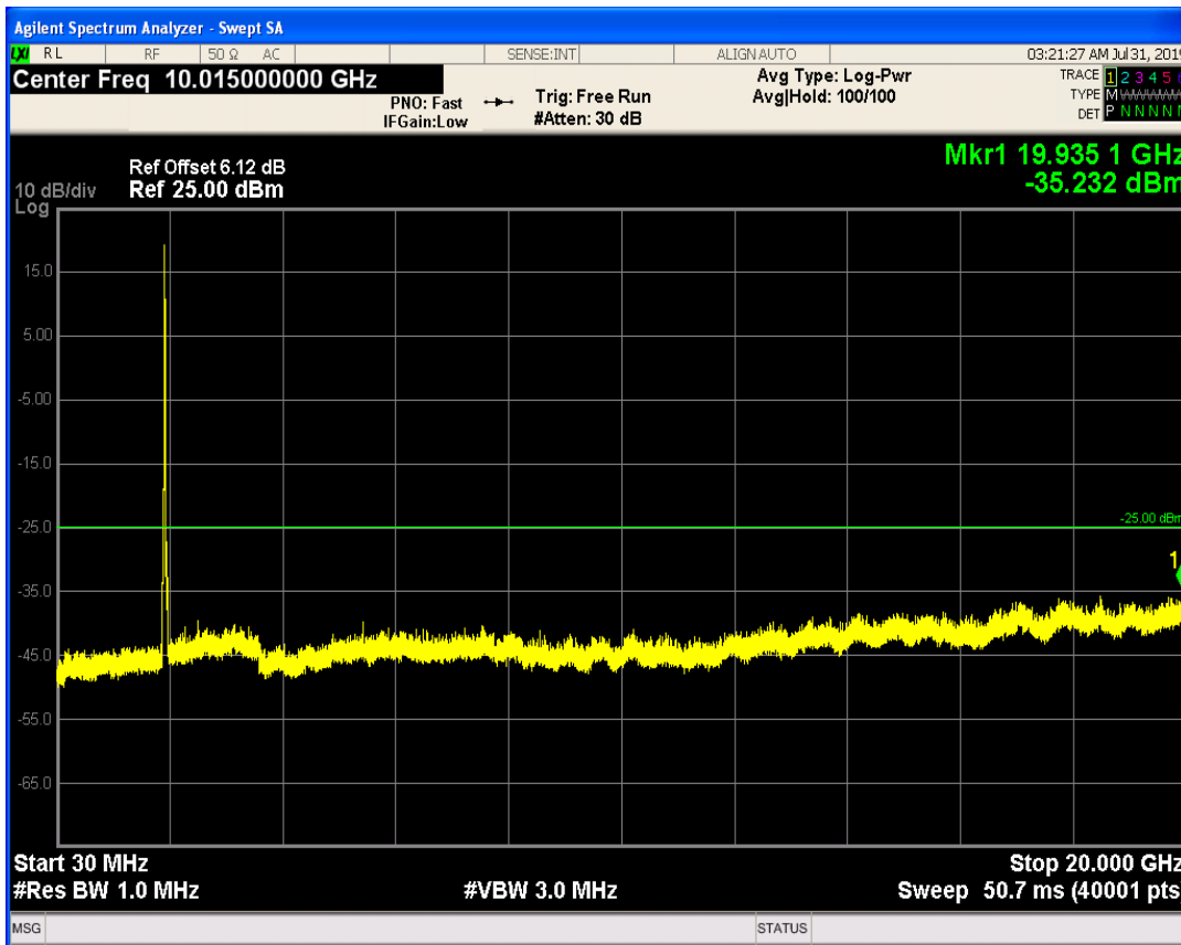
LTE Band1 QPSK BW=15MHz Channel=18525 RB Size=75 Position=#0
