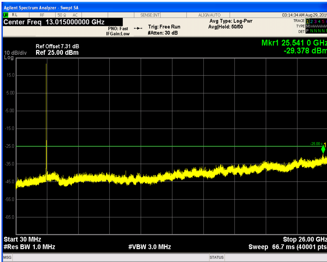
LTE Band41 QPSK BW=5MHz Channel=41165 RB Size=25 Position=#0
