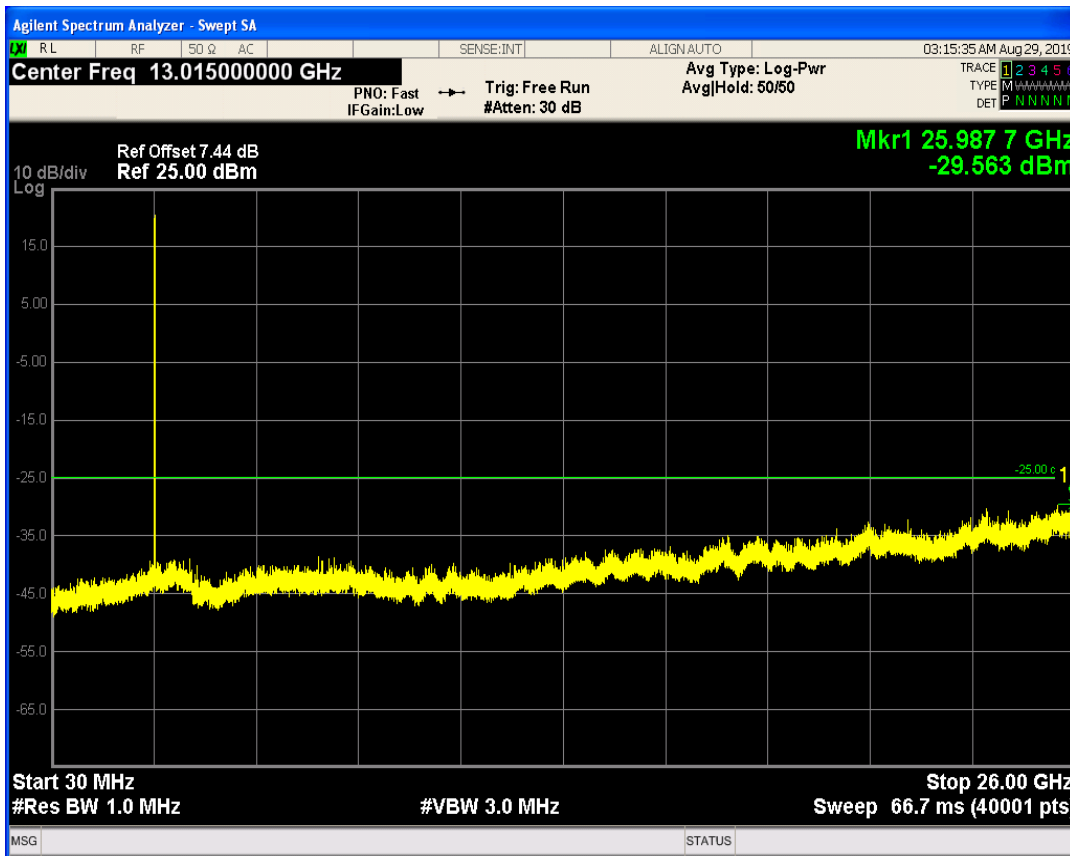
LTE Band41 QPSK BW=10MHz Channel=40290 RB Size=50 Position=#0
