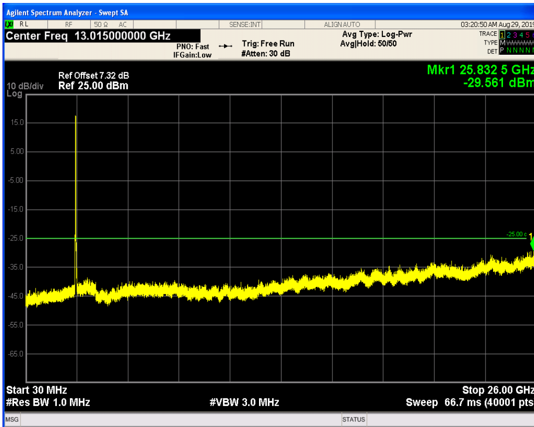
LTE Band41 QPSK BW=20MHz Channel=41090 RB Size=100 Position=#0
