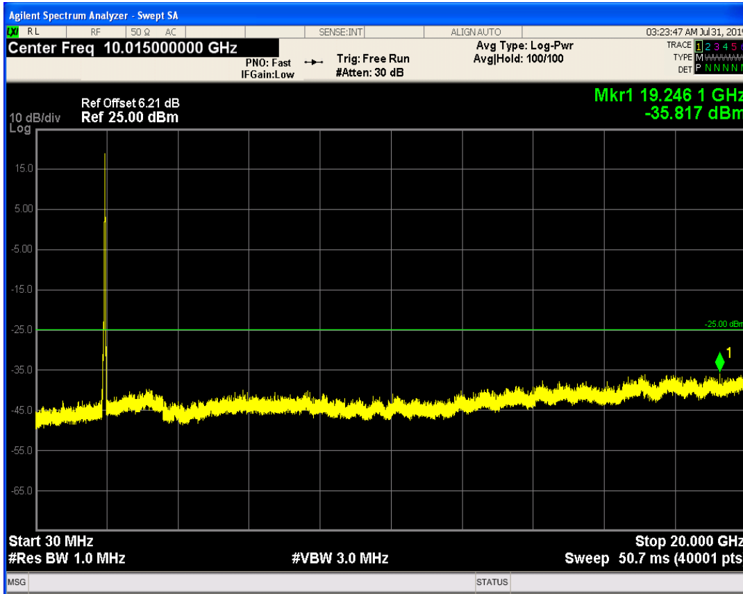
LTE Band1 QAM16 BW=20MHz Channel=18100 RB Size=100 Position=#0
