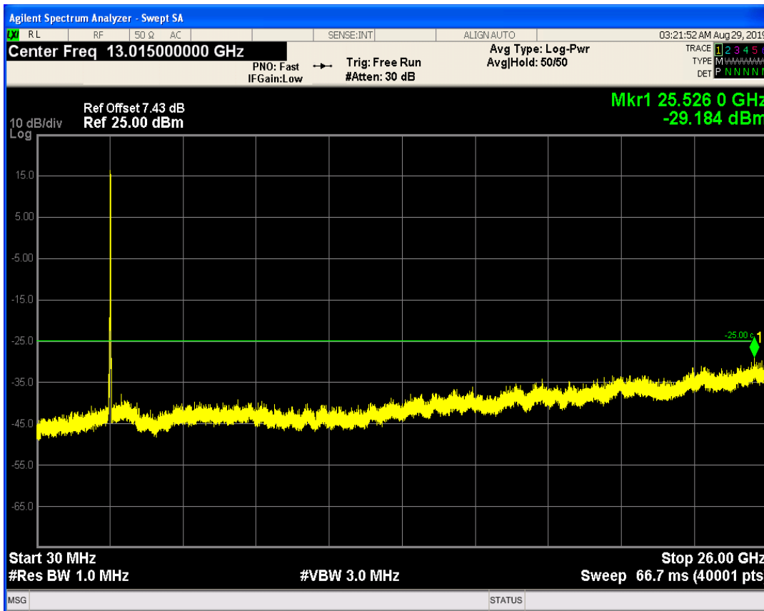
LTE Band41 QAM16 BW=20MHz Channel=41090 RB Size=100 Position=#0
