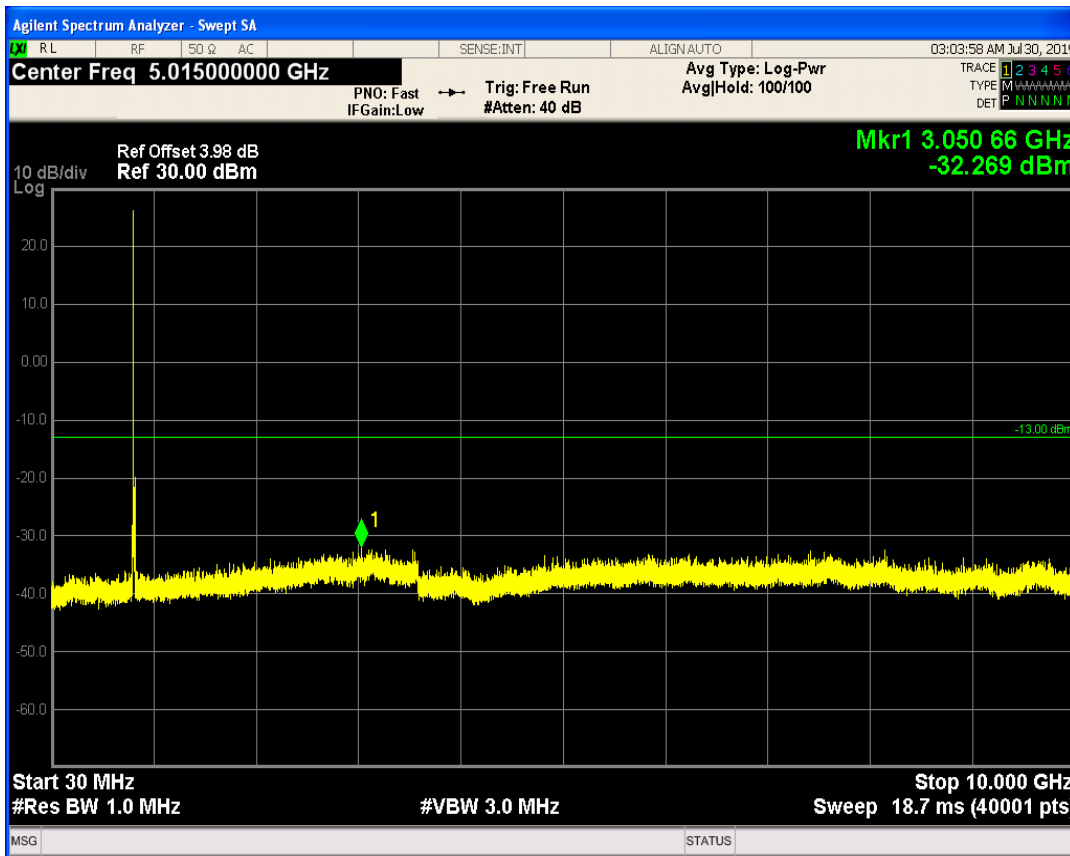
LTE Band1 QPSK BW=10MHz Channel=18550 RB Size=50 Position=#0
