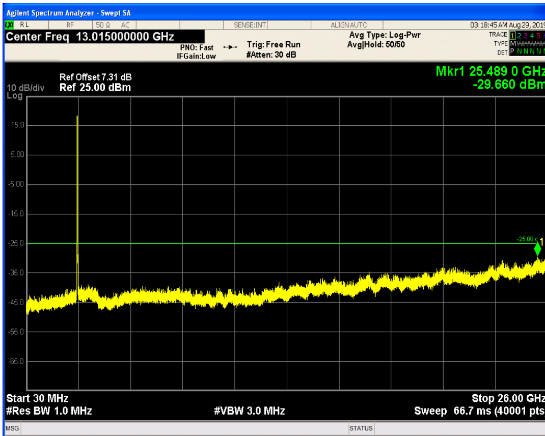
LTE Band41 QAM16 BW=15MHz Channel=41115 RB Size=75 Position=#0
