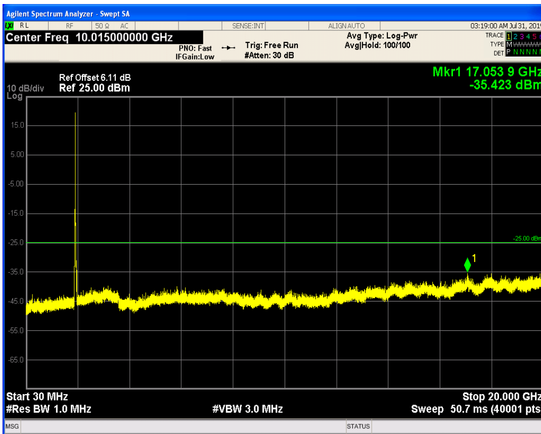
LTE Band1 QAM16 BW=10MHz Channel=18550 RB Size=50 Position=#0
