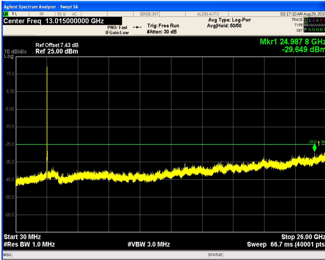
LTE Band41 QAM16 BW=10MHz Channel=41140 RB Size=50 Position=#0
