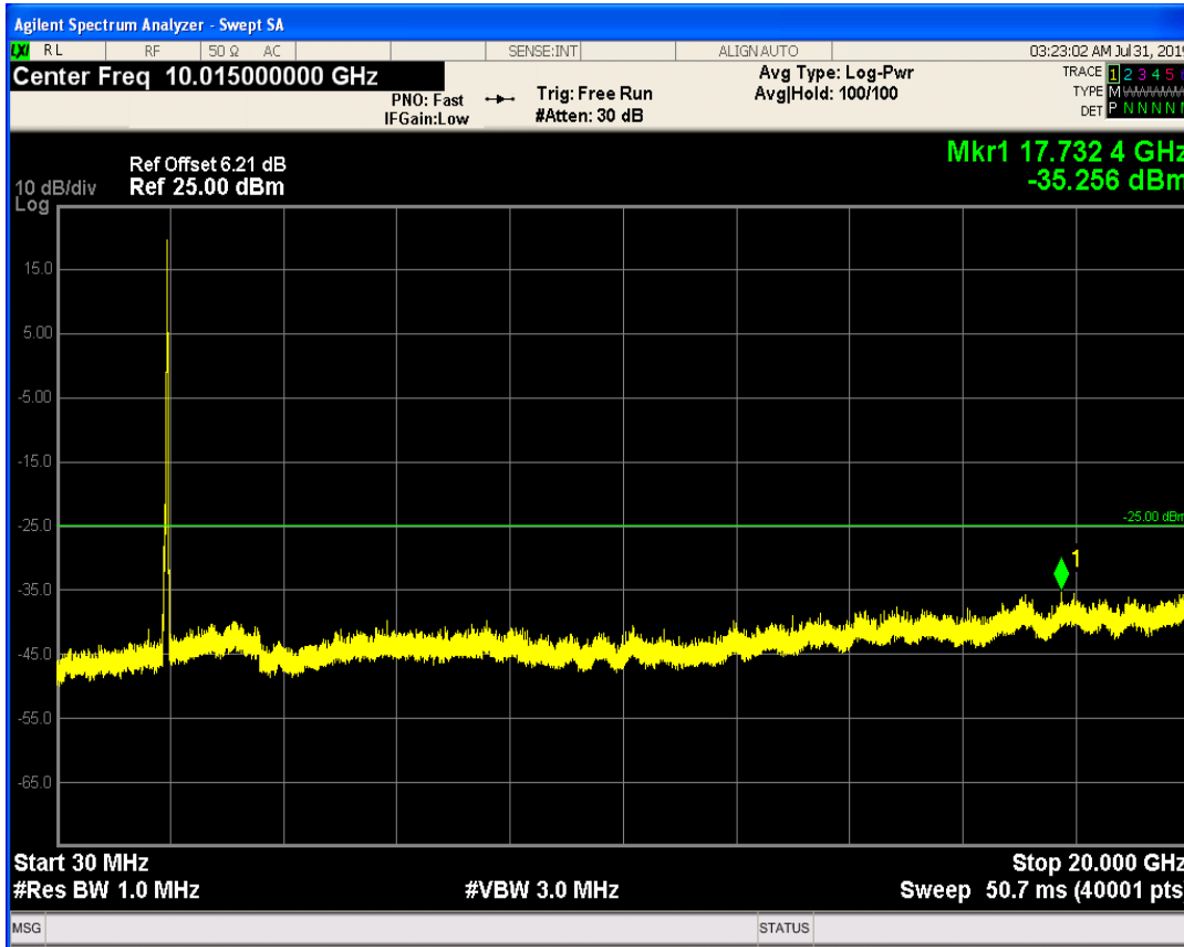
LTE Band1 QPSK BW=20MHz Channel=18100 RB Size=100 Position=#0
