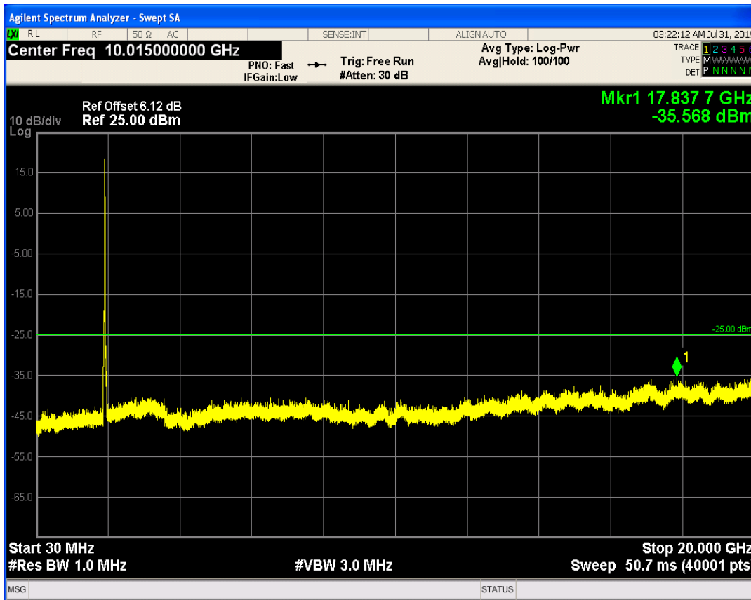
LTE Band1 QPSK BW=5MHz Channel=18575 RB Size=25 Position=#0
