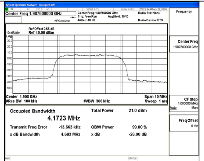
Channel 9538 / 1907.6 MHz
