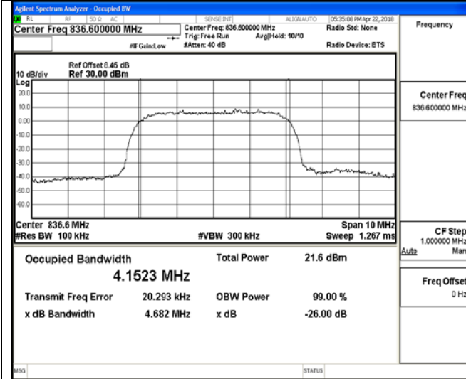
Channel 4183 / 836.6 MHz
