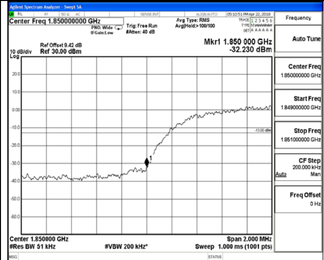
Channel 9262 / 1852.4 MHz
