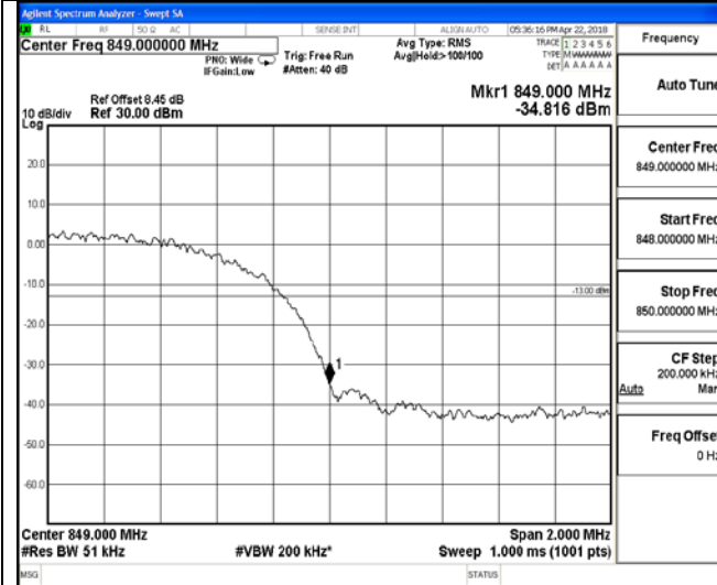
Channel 4233 / 846.6 MHz
