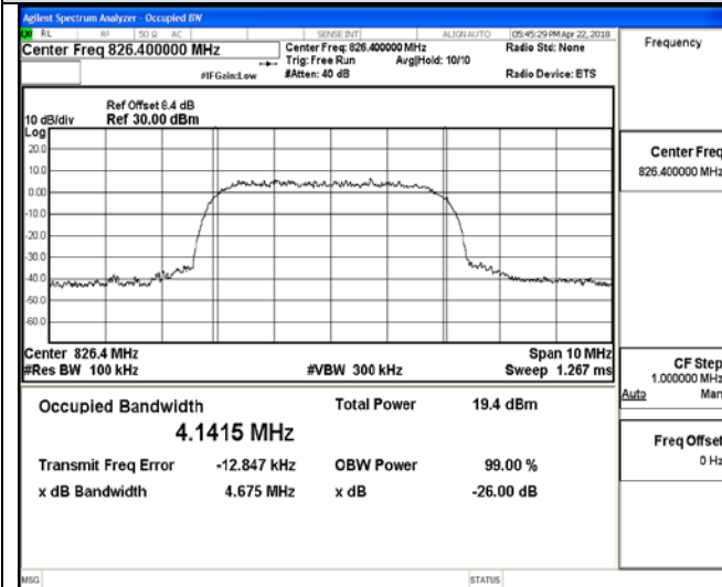
Channel 4132 / 826.4 MHz
