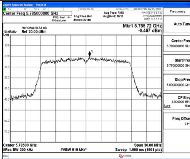
Channel 157 / 5785 MHz
