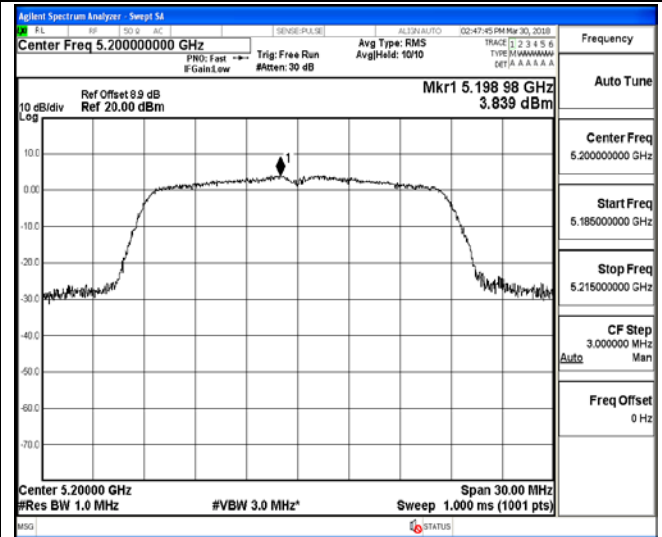
Channel 40 / 5200 MHz
