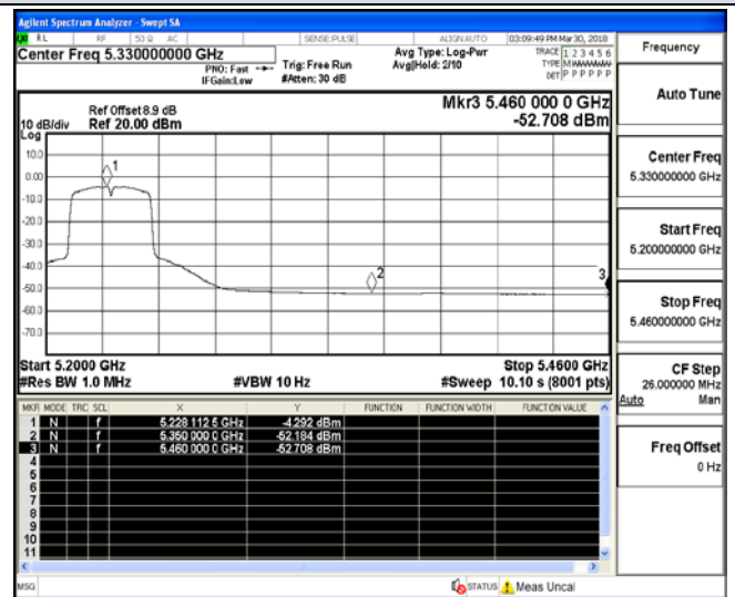
Channel 46 / 5230 MHz – Average
