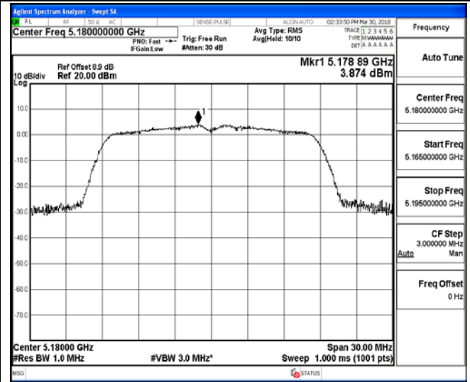
Channel 36 / 5180 MHz
