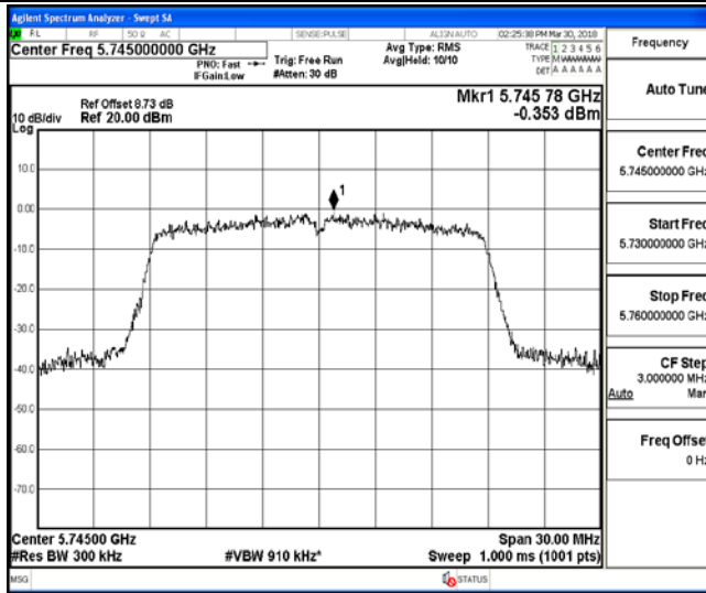
Channel 149 / 5745 MHz
