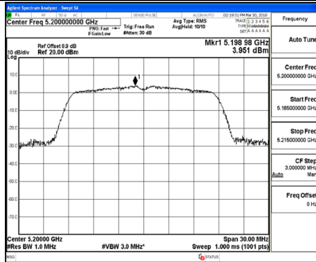
Channel 40 / 5200 MHz
