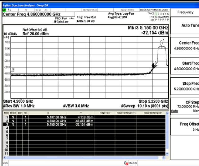
Channel 38 / 5190 MHz – Peak
