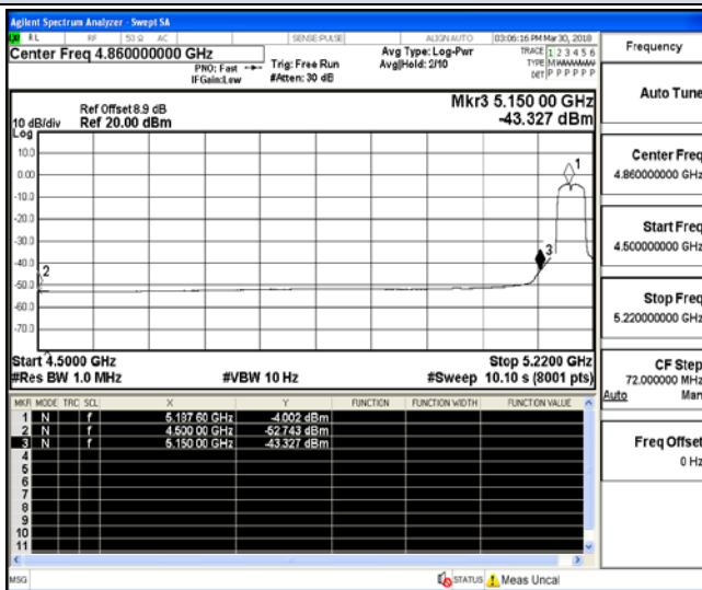
Channel 38 / 5190 MHz – Average
