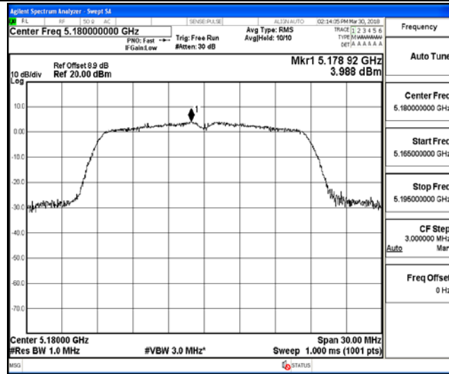
Channel 36 / 5180 MHz
