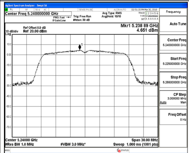
Channel 48 / 5240 MHz
