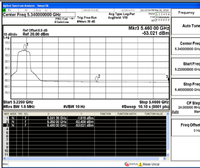
Channel 48 / 5240 MHz – Average
