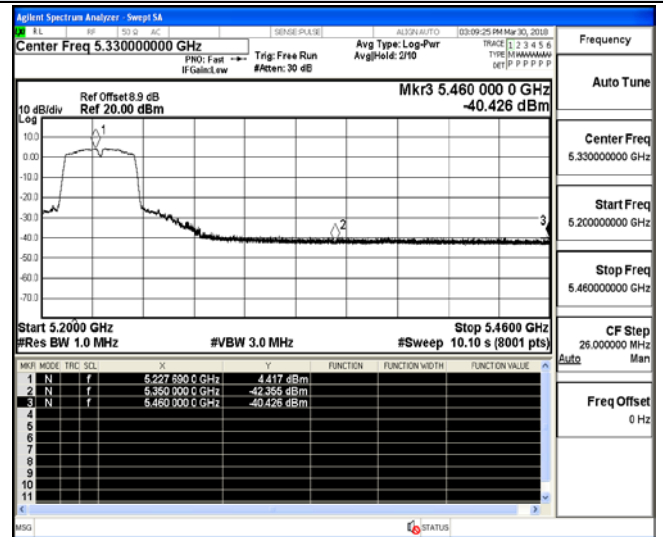
Channel 46 / 5230 MHz – Peak
