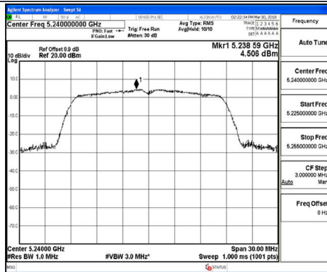
Channel 48 / 5240 MHz
