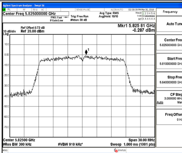
Channel 165 / 5825 MHz
