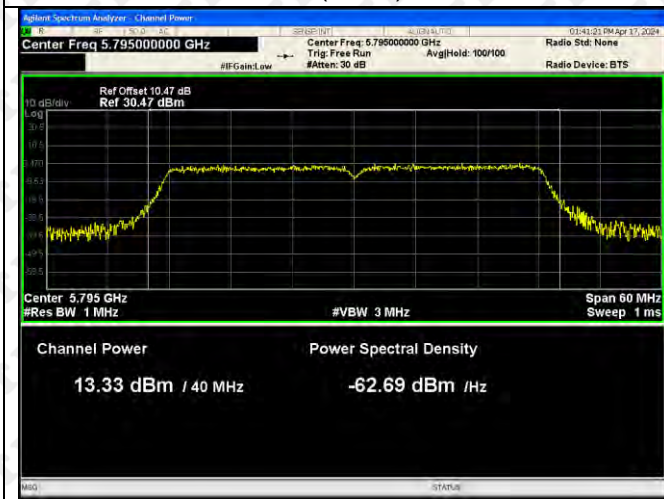
802.11ax(VH40)-5795
