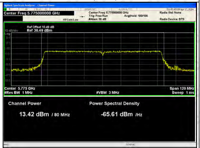
802.11ax(VH80)-5775
