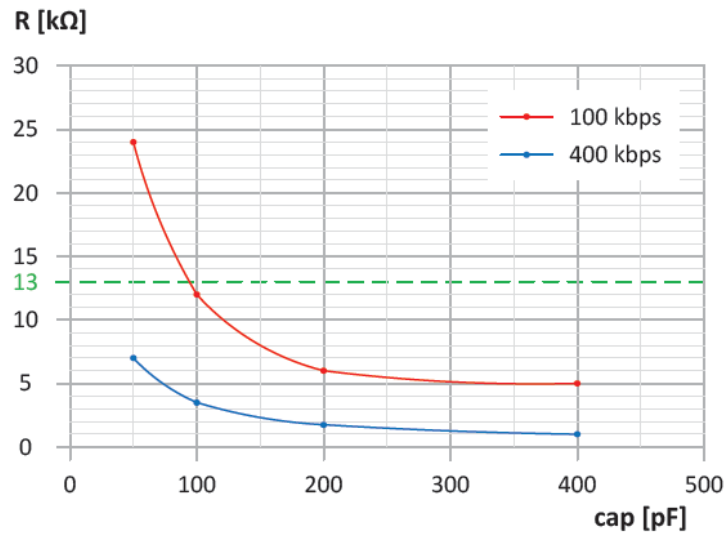
Recommended TWIM pullup value vs. line capacitance
