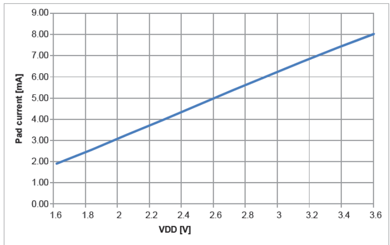
Max sink current vs Voltage, standard drive
