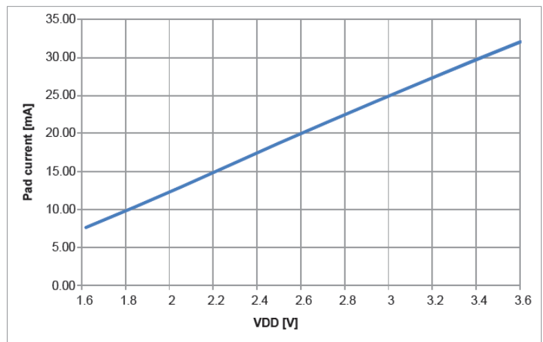
Max sink current vs Voltage, high drive
