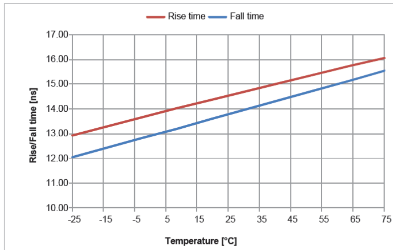
Rise and fall time vs Temperature, 10%-90%, 25pF load capacitance, VDD = 3.0 V
