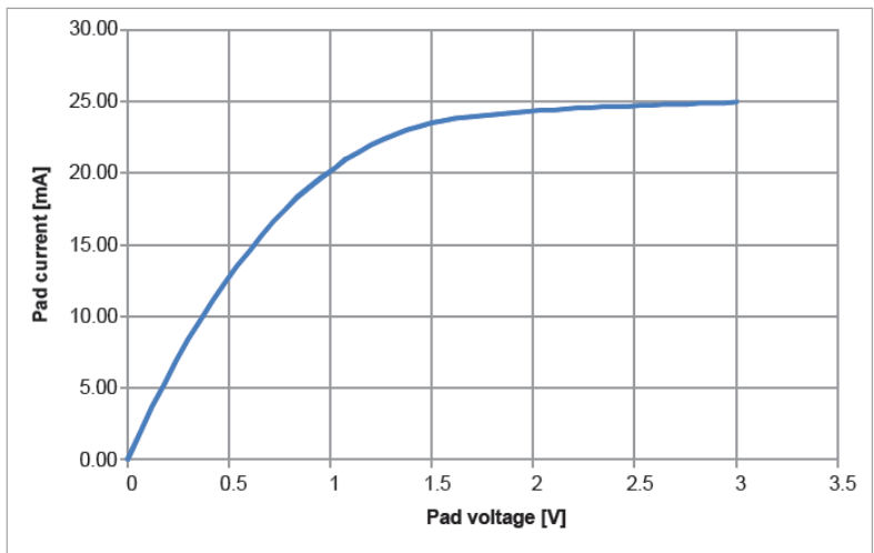
GPIO drive strength vs Voltage, high drive, VDD = 3.0 V
