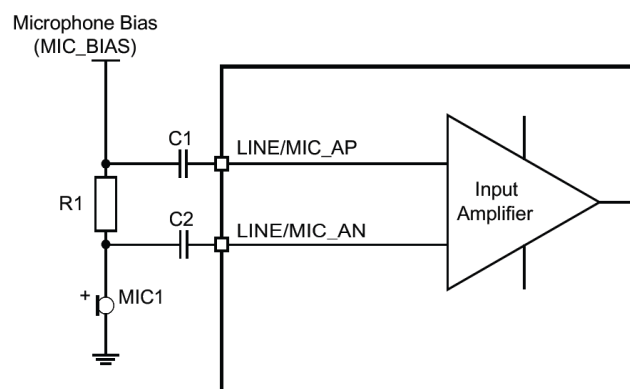
Figure 12: Microphone Biasing
