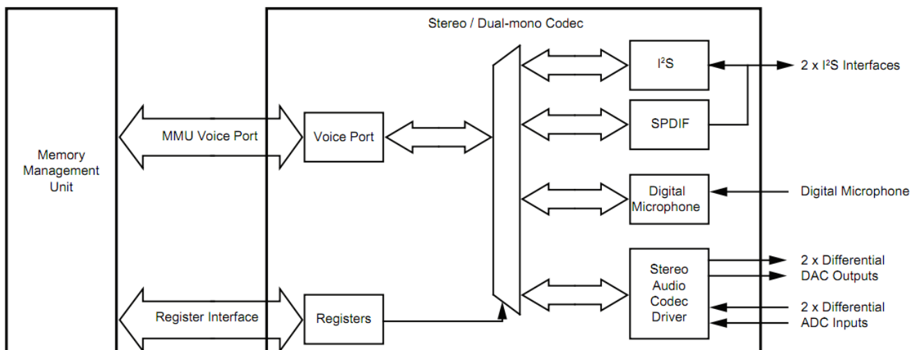
Figure 9: Audio Interface
