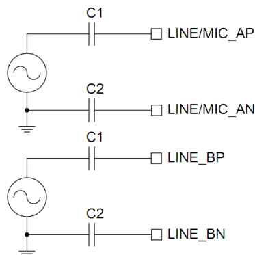
Figure 14: Single-ended Input
