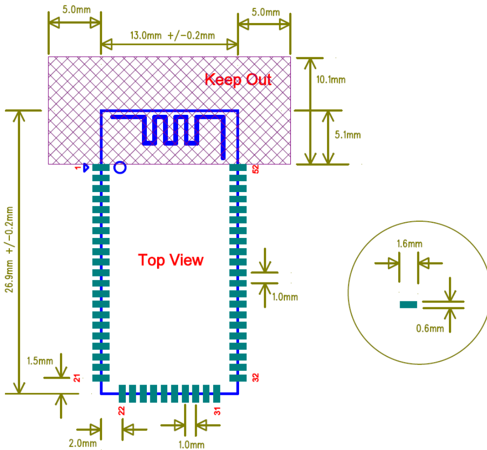
Figure 3: FSC-BT1026 footprint
