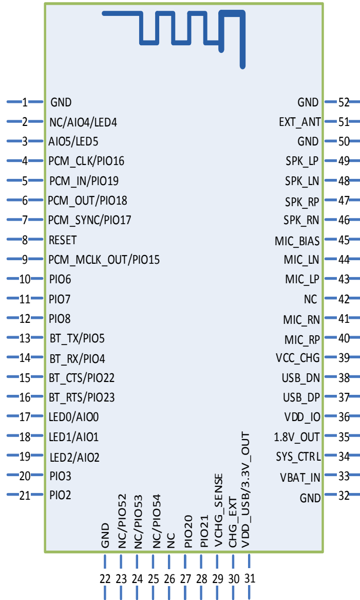
Figure 2: FSC-BT1026x PIN Diagram(Top View)
