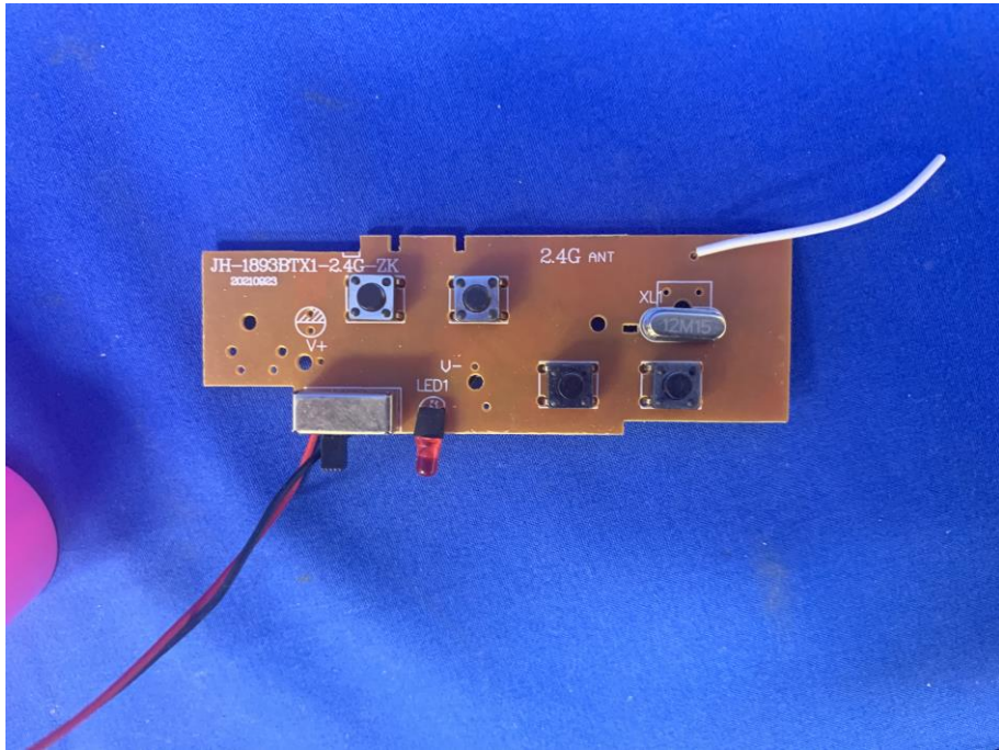
antenna length: 3.8cm
