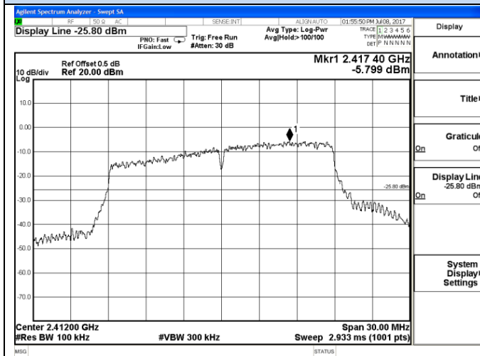
IEEE 802.11n HT20-Channel 1 / 2412 MHz
