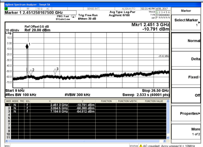
802.11n-HT40-High channel
