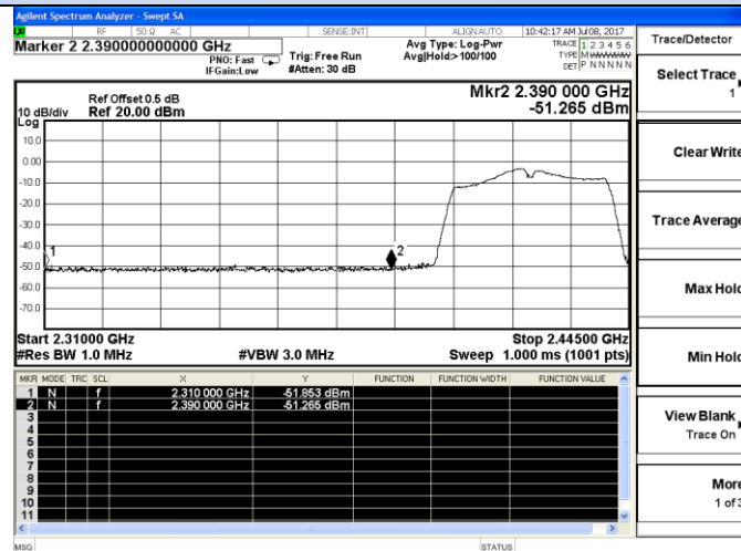
802.11n-HT40-Low channel(Peak)
