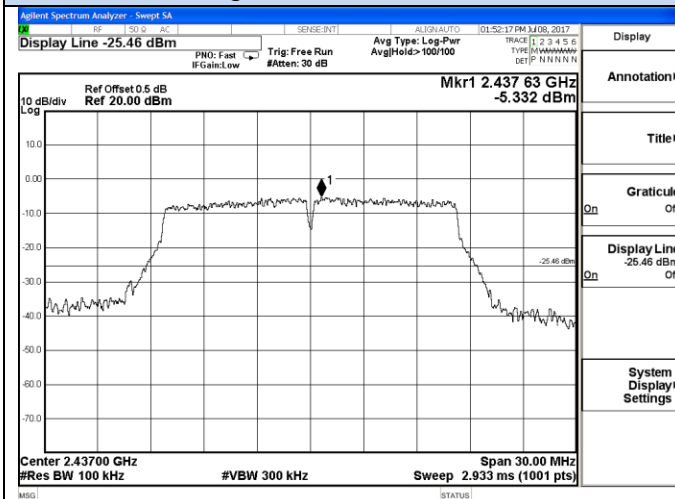
802.11g-Middle channel Reference
