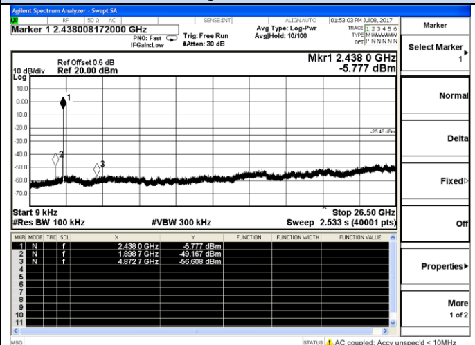
802.11g-Middle channel
