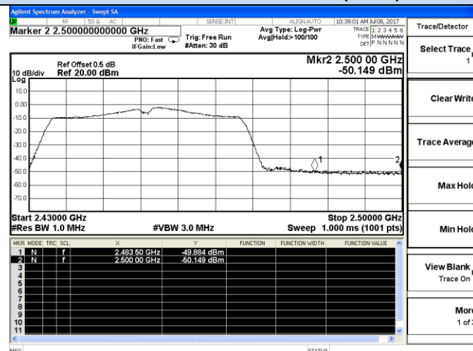
802.11n-HT40-High channel(Peak)
