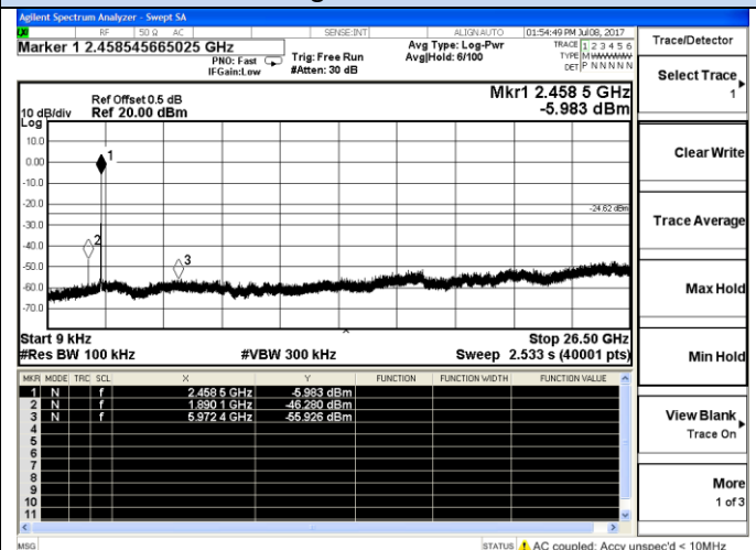
802.11g-High channel
