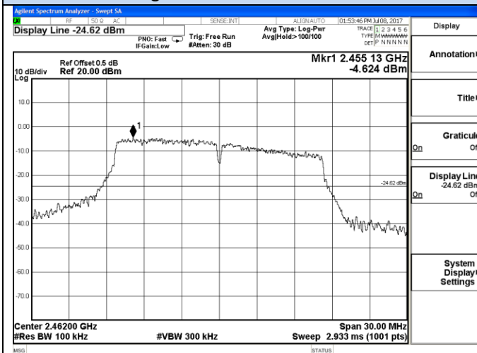
802.11g-High channel Reference
