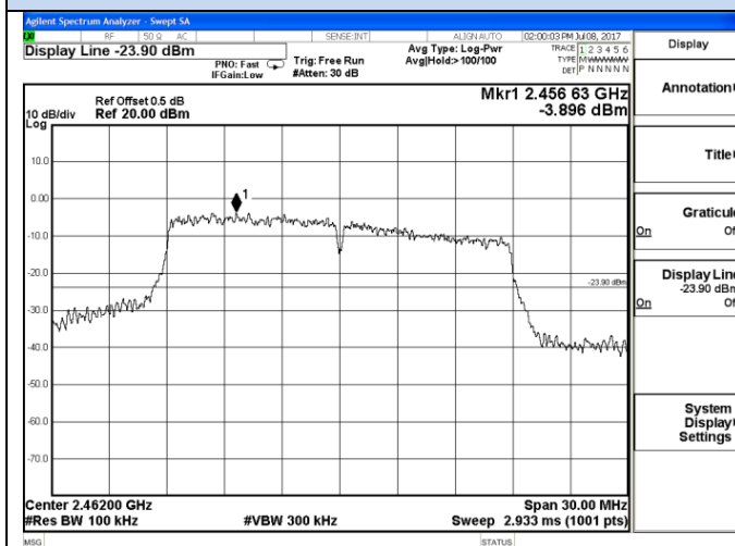
IEEE 802.11n HT20-Channel 11 / 2462 MHz
