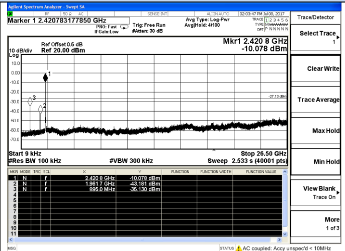
802.11n-HT40-Low channel
