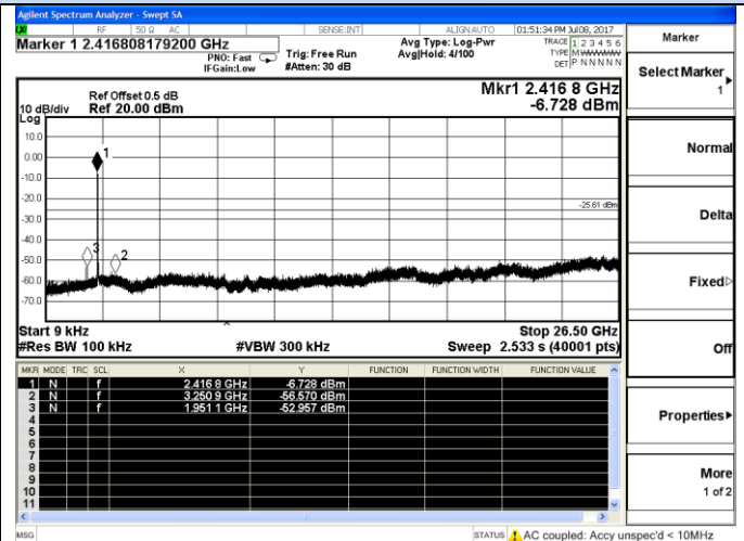
802.11g-Low channel
