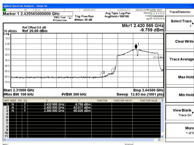
802.11n-HT40-Low channel
