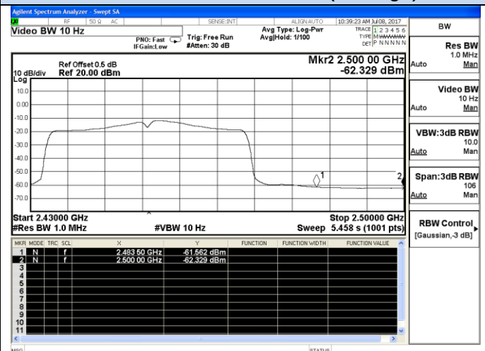
802.11n-HT40-High channel(Average)
