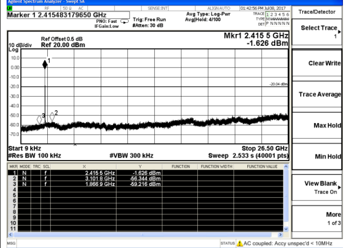
802.11b-Low channel
