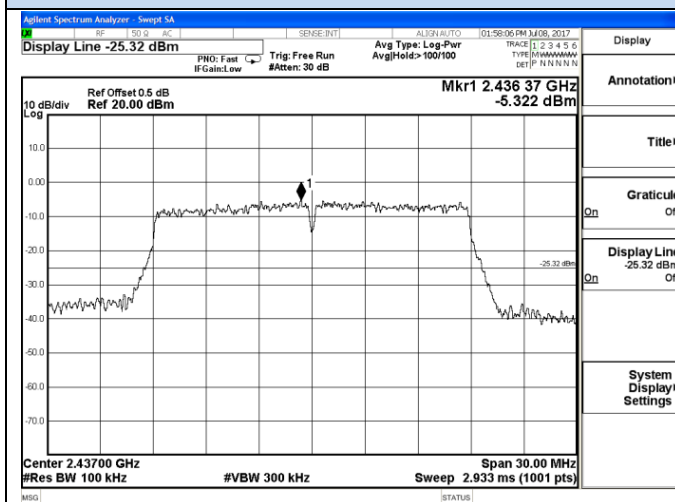
IEEE 802.11n HT20-Channel 6 / 2437 MHz
