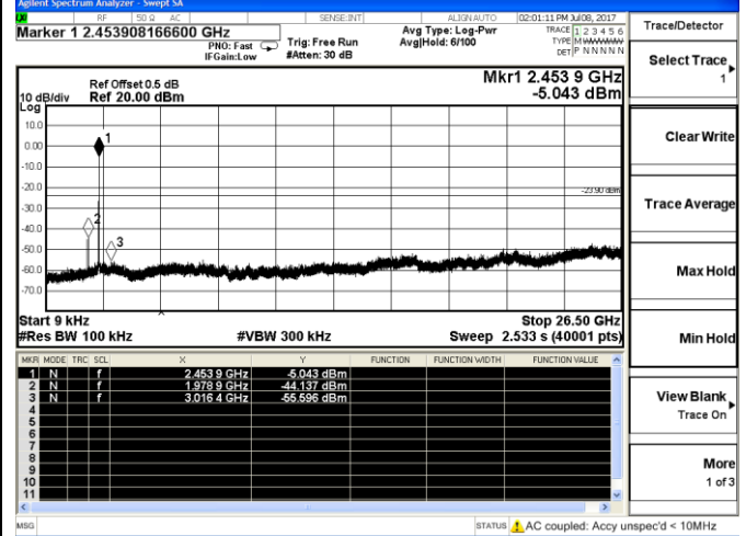
802.11n-HT20-Middle channel
