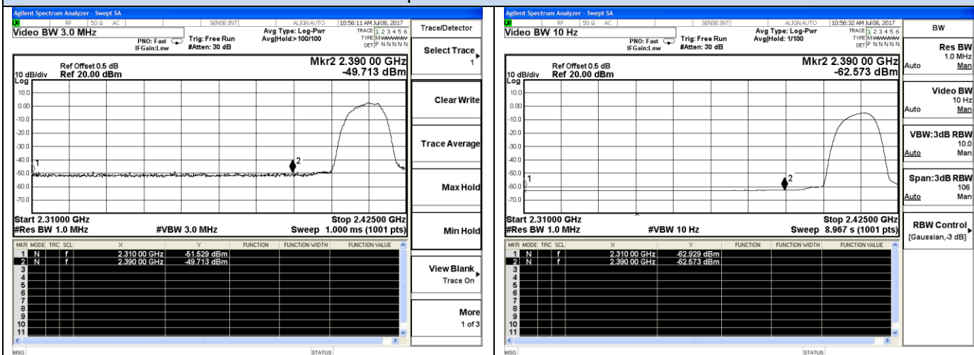
802.11b-Low channel(Peak)
