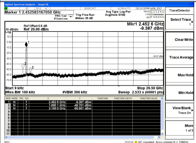
802.11n-HT40-Middle channel
