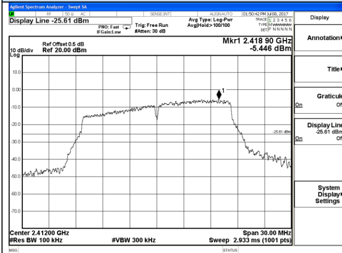
802.11g-Low channel Reference
