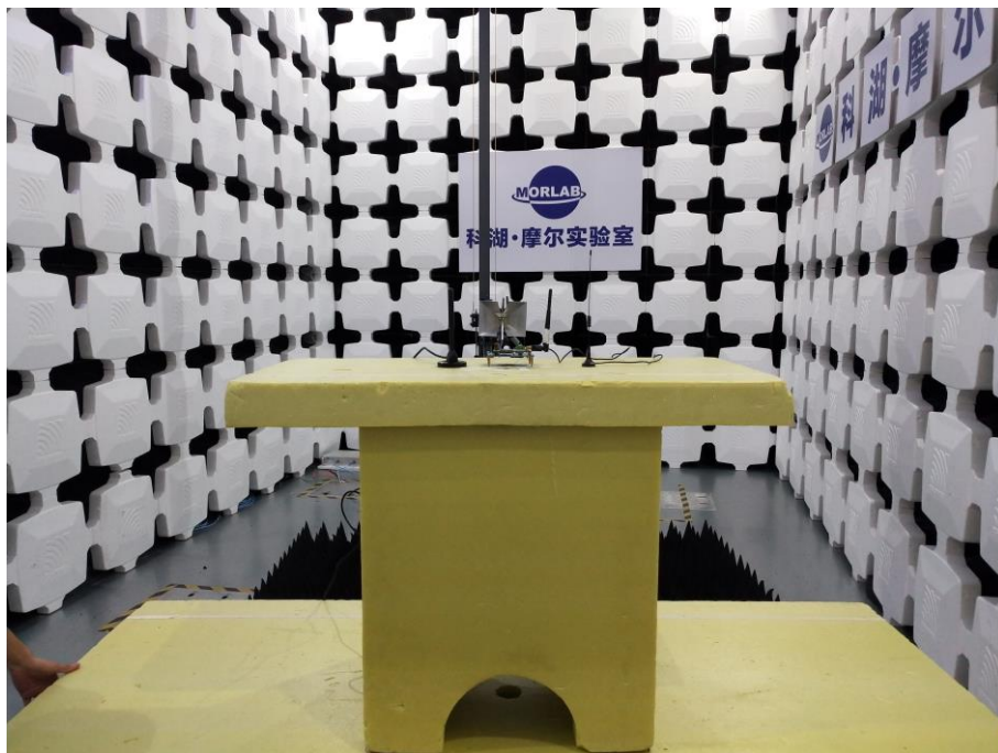
RE Above 1G_ WWAN Link + WiFi Link
