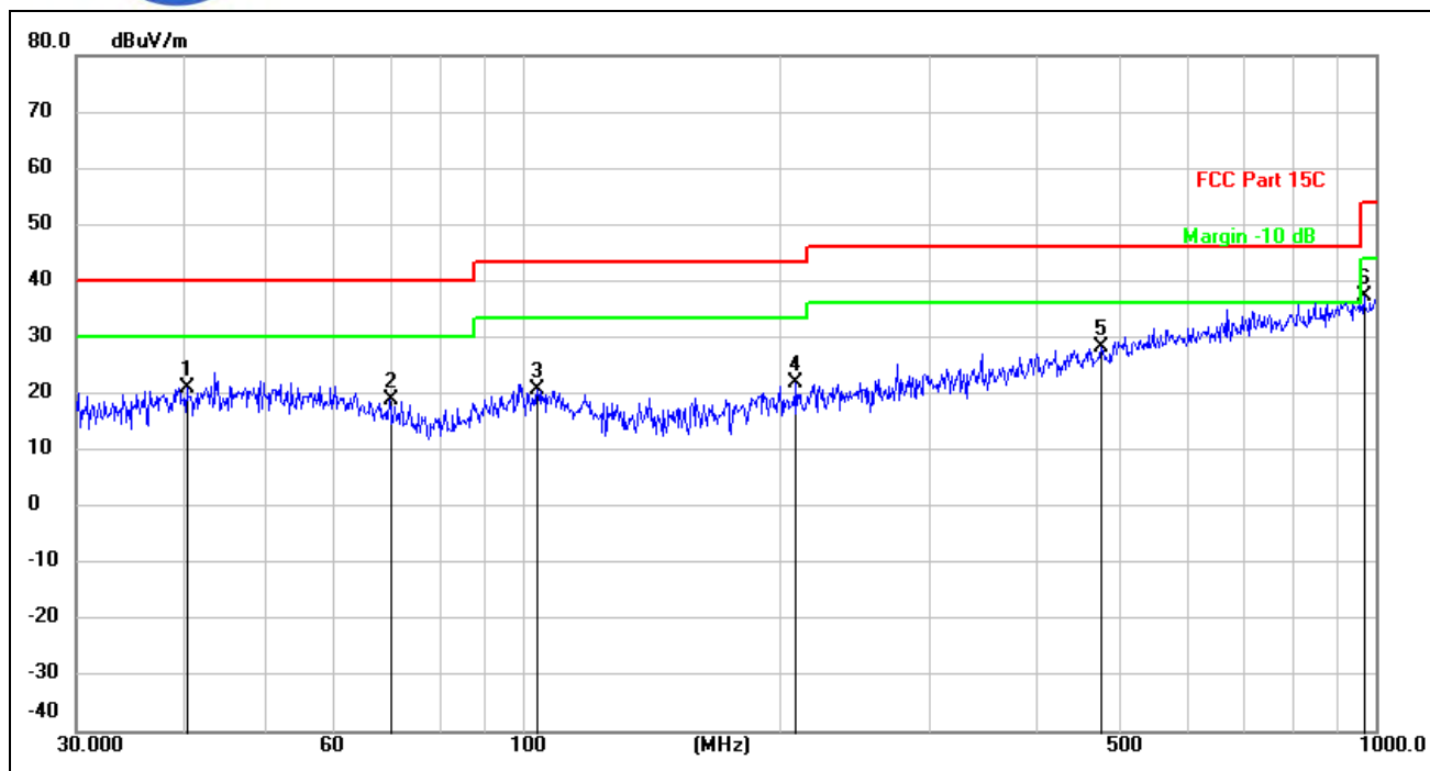
(802.11 n20 _2437MHz, Antenna Horizontal, 30MHz to 1GHz)
