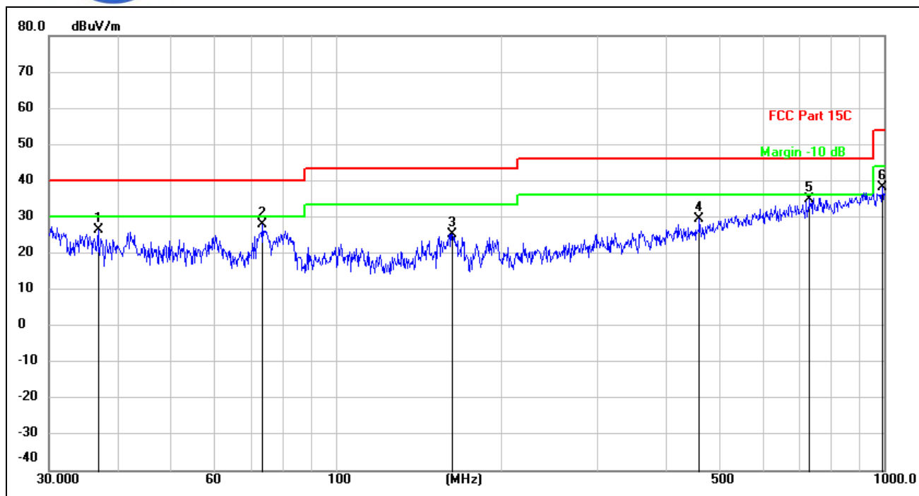
(802.11 n20 _2412MHz, Antenna Vertical, 30MHz to 1GHz)
