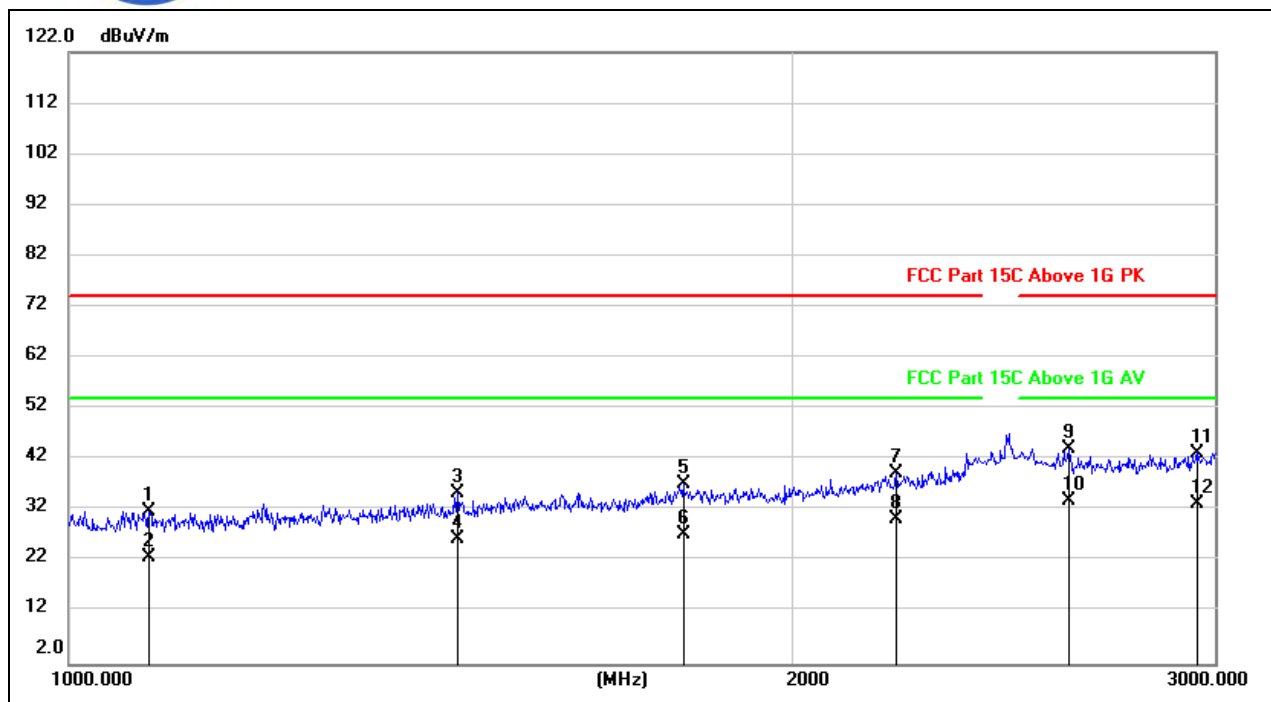
(802.11 n40 _2422MHz, Antenna Horizontal, 1GHz to 3GHz)
