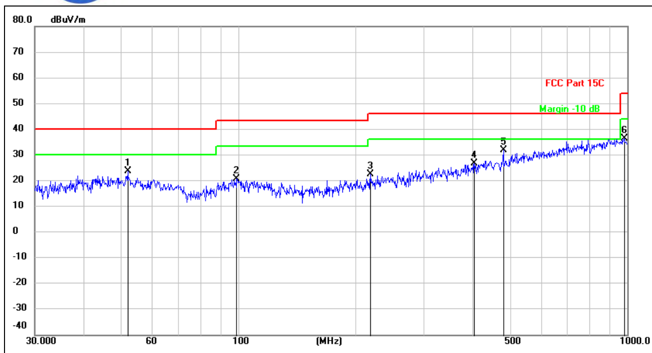
(802.11 n20 _2437MHz, Antenna Vertical, 30MHz to 1GHz)
