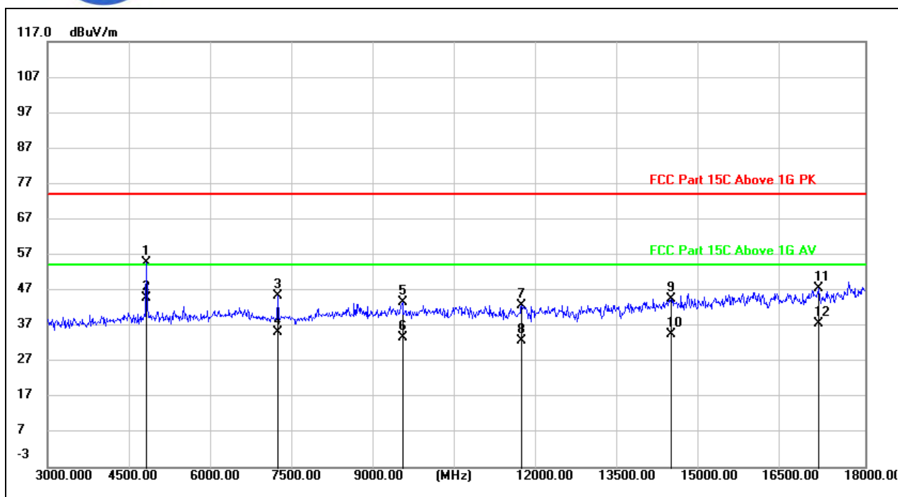
(802.11 n20 _2412MHz, Antenna Vertical, 3GHz to 18GHz)
