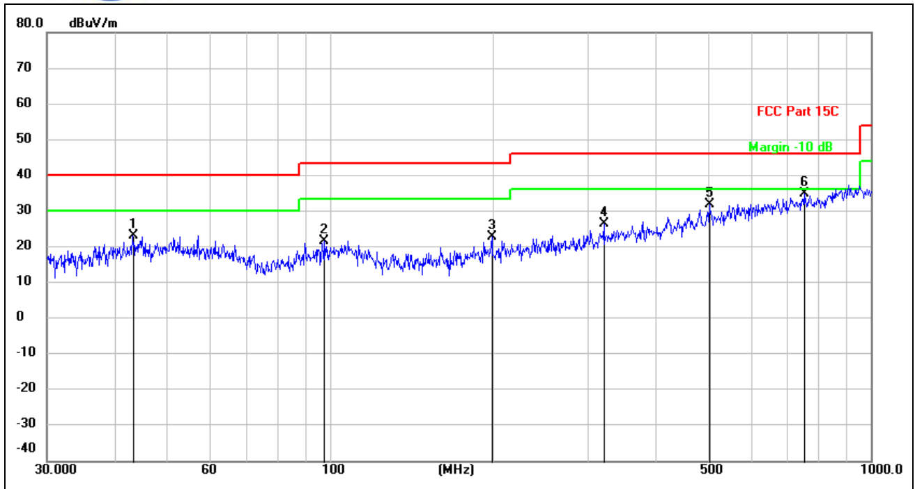
(802.11 n40 _2437MHz, Antenna Horizontal, 30MHz to 1GHz)
