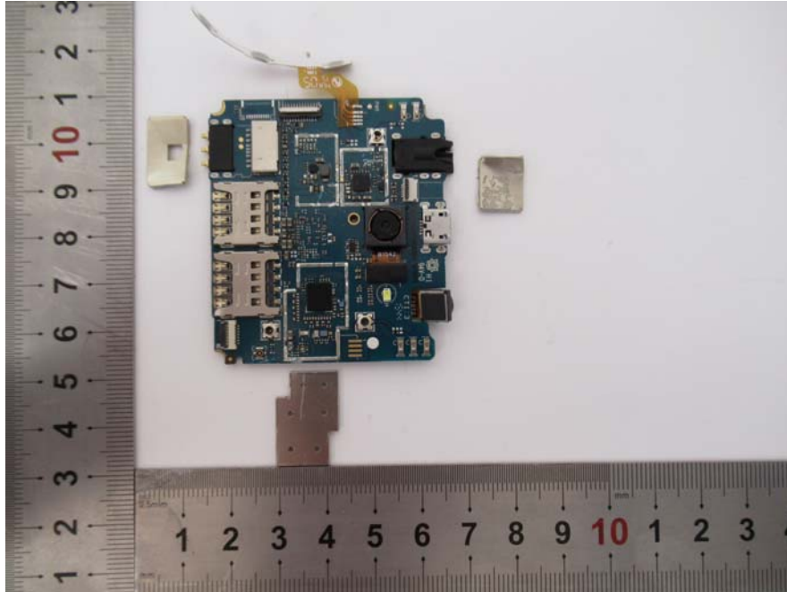
EUT – PCB-2 Shielding off Bottom View
