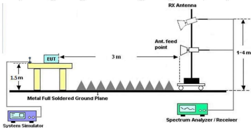
Figure 3. Above 1 GHz
