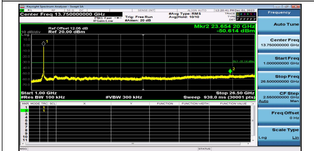
11N40SISO_Ant1_2422_1000~26500
