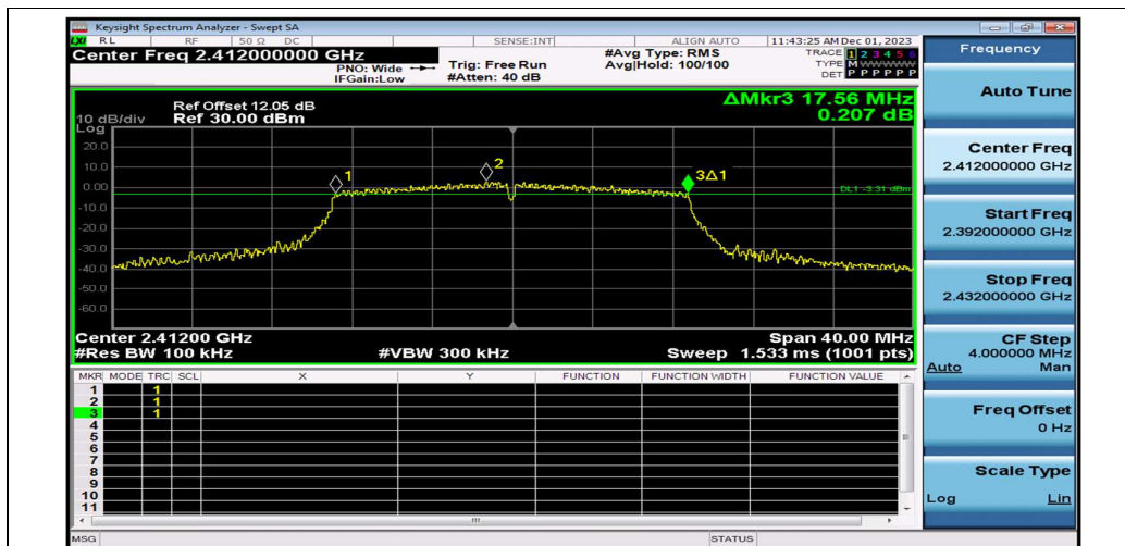
11N20SISO_Ant1_2412
