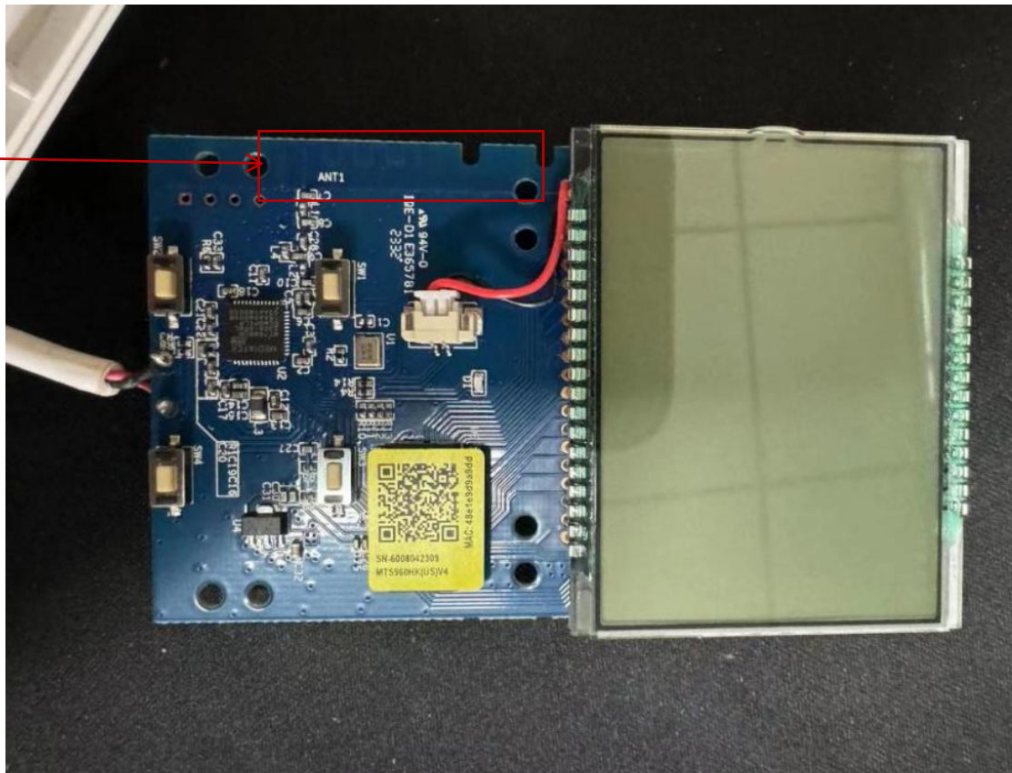
PCB Antenna
