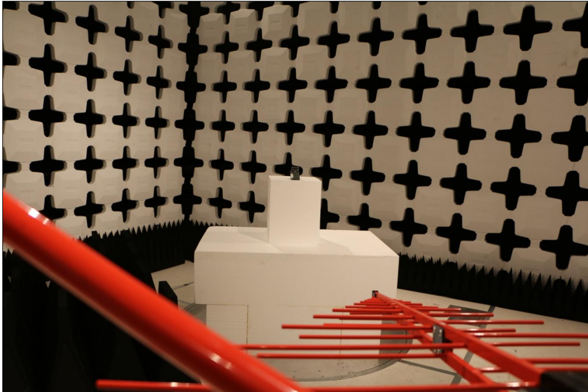
Radiated Emissions < 1 GHz
