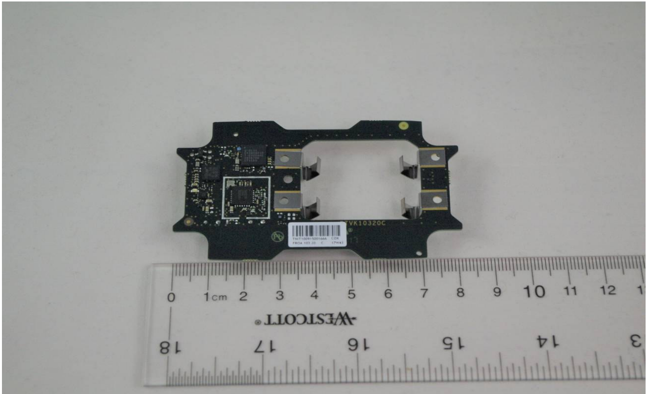
TNIT100-915-Inside_Top_No_Shield
