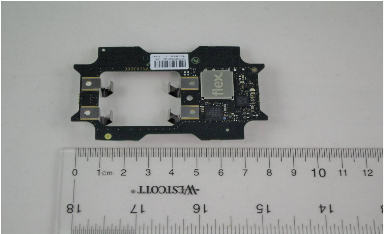
TNIT100-915-Inside_Top
