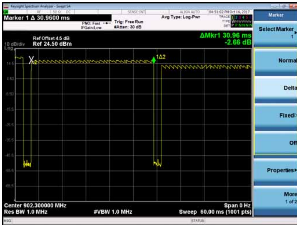
Channel 31 (902.3MHz)
