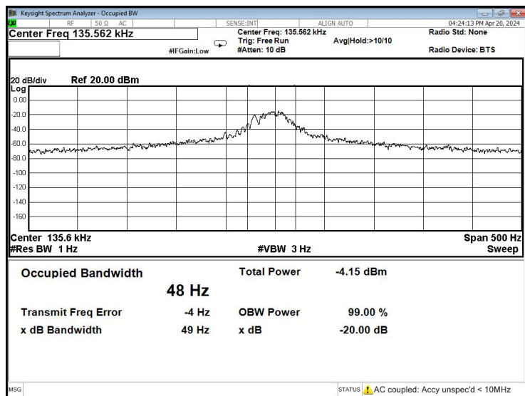
Test plot of 99% and 20 dB Bandwidth Measurement
