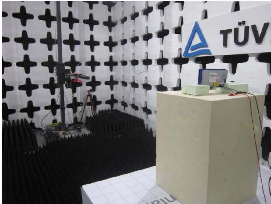
Set-up 1÷18GHz
