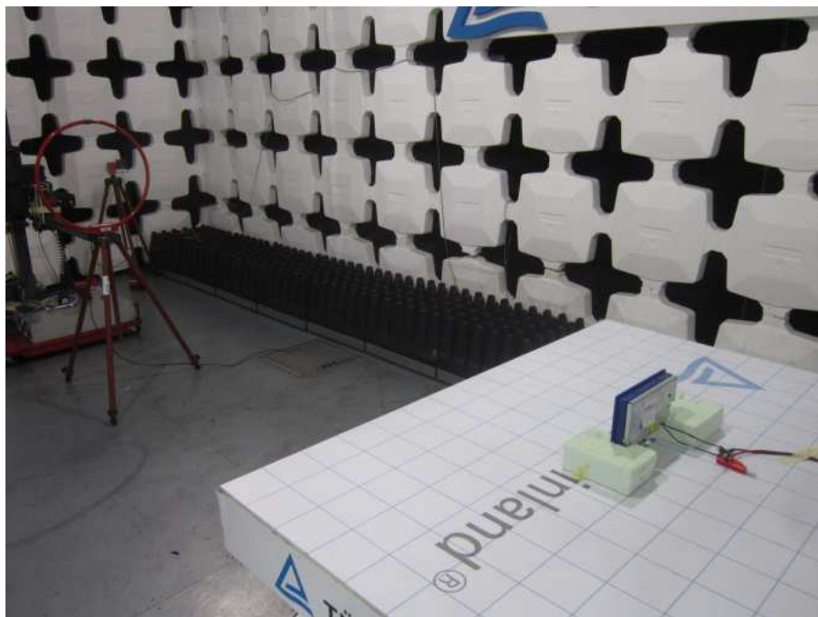
Set-up 9KHz-30MHz
