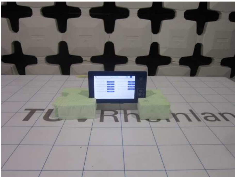
Set-up 30MHz-1GHz
