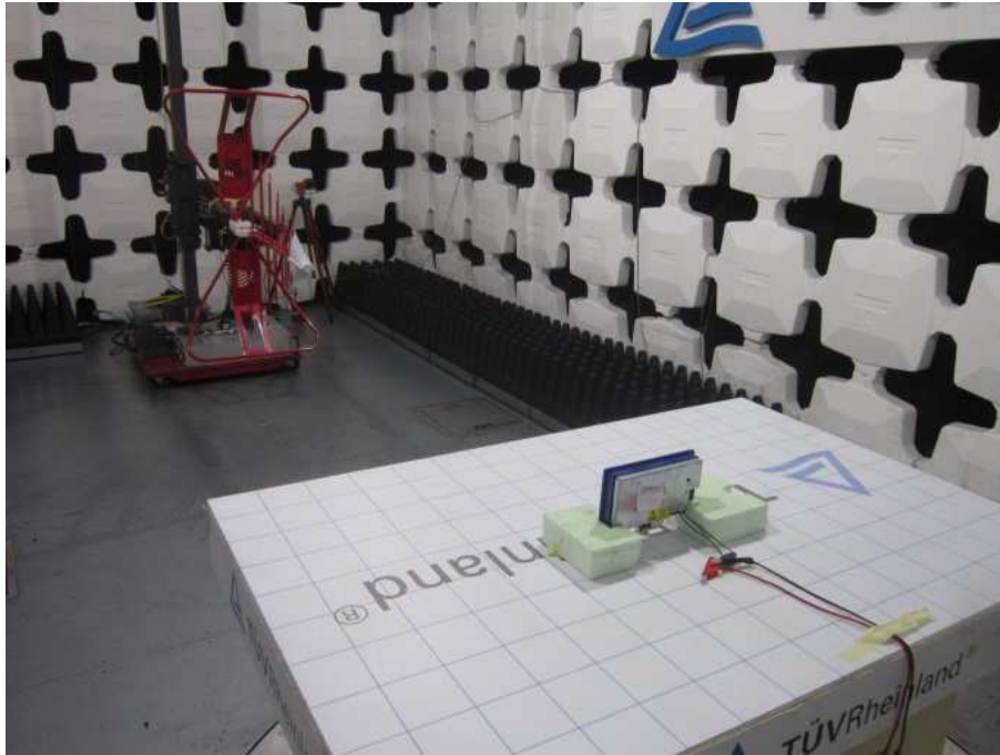
Set-up 30MHz-1GHz
