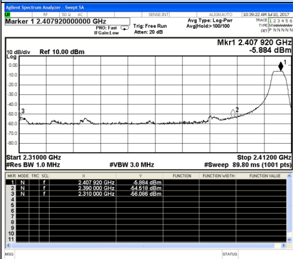
2407 MHz - Peak
