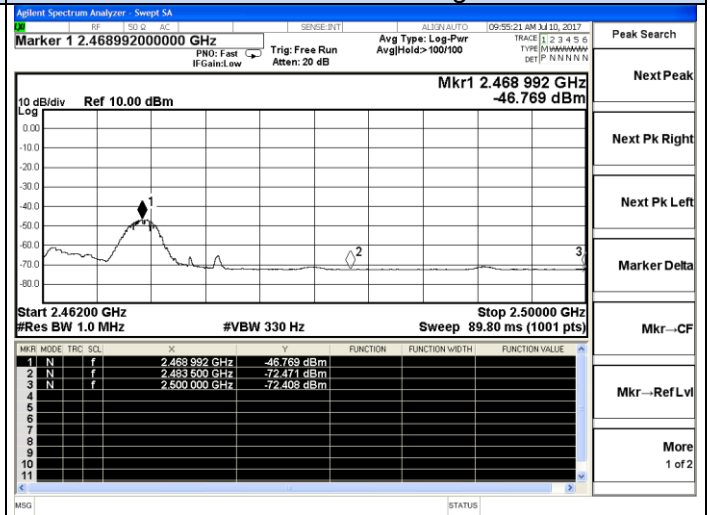
2469 MHz - Average
