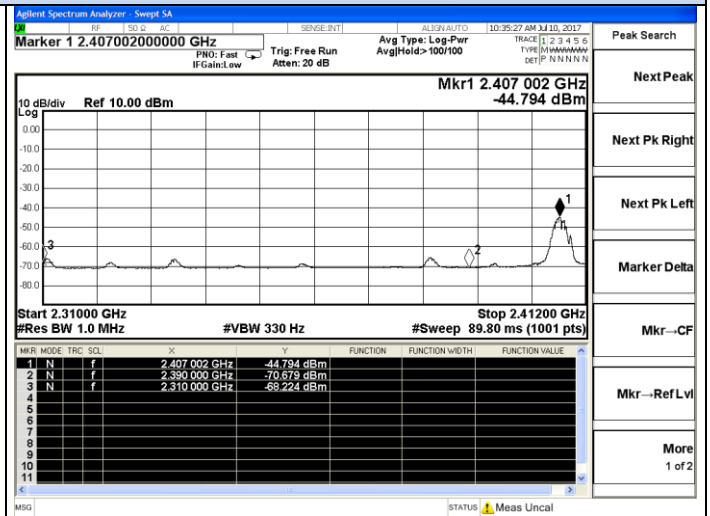
2407 MHz - Average
