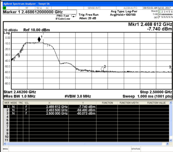
2469 MHz - Peak
