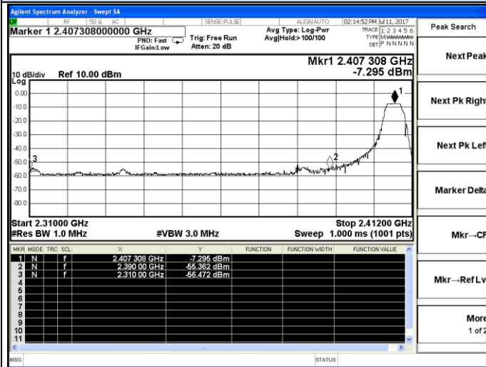
2407 MHz – Peak
