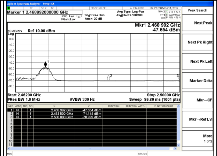
2469 MHz – Average
