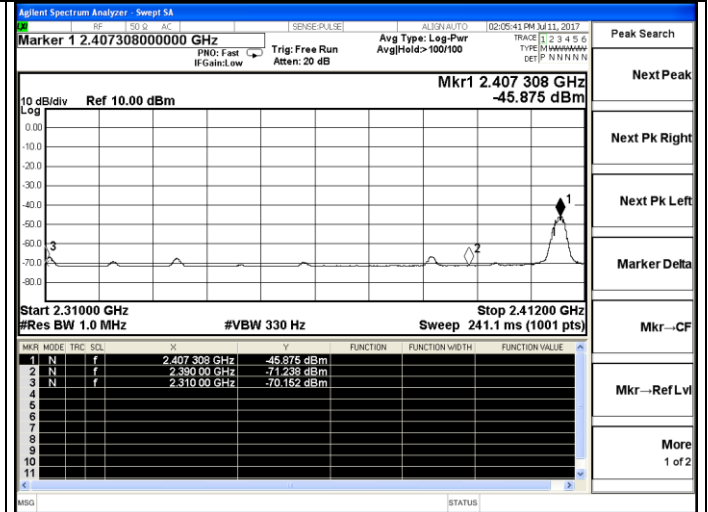
2407 MHz - Average
