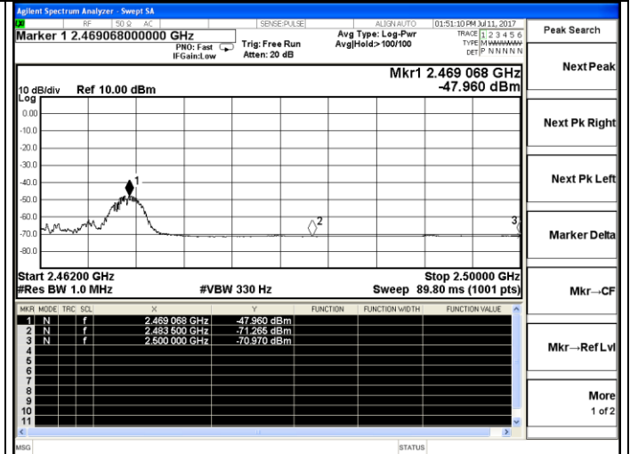
2469 MHz - Average
