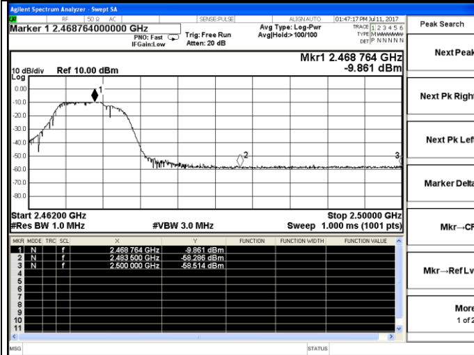
2469 MHz - Peak
