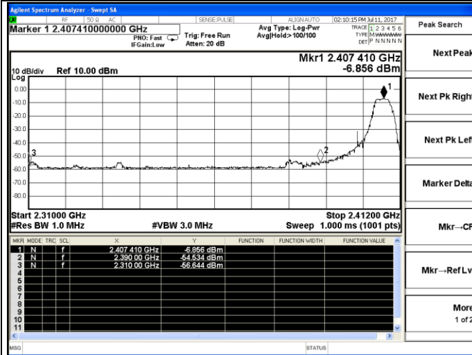
2407 MHz - Peak
