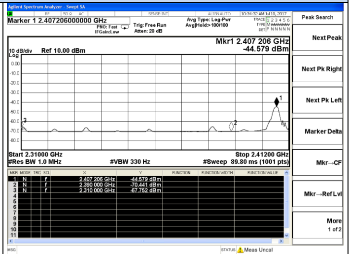
2407 MHz – Average
