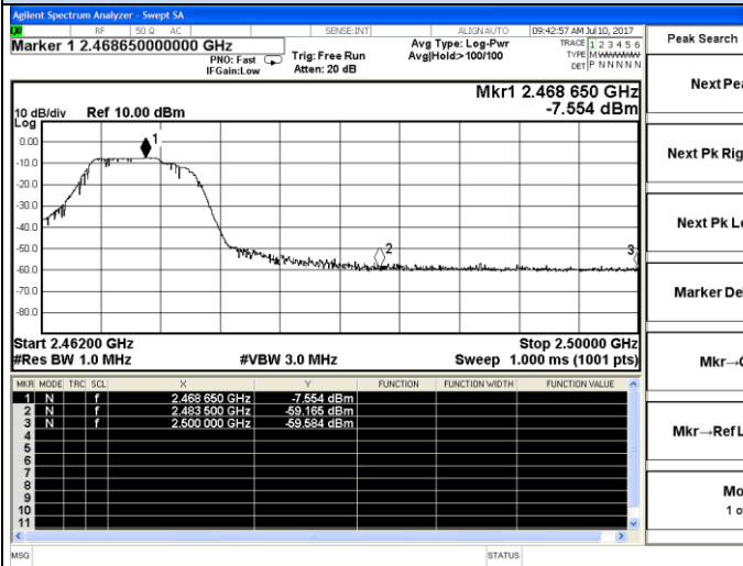
2469 MHz – Peak
