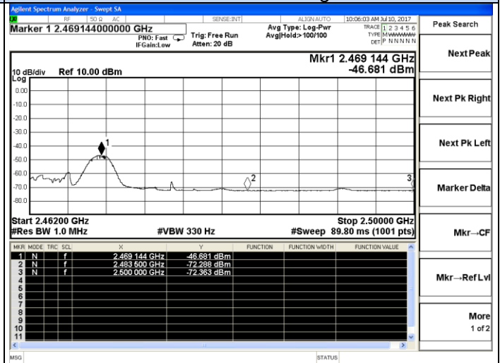
2469 MHz – Average
